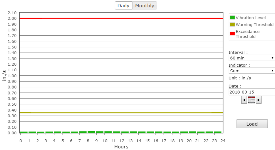
Figure 20: North Vibration Monitor VM-1 on Thursday
