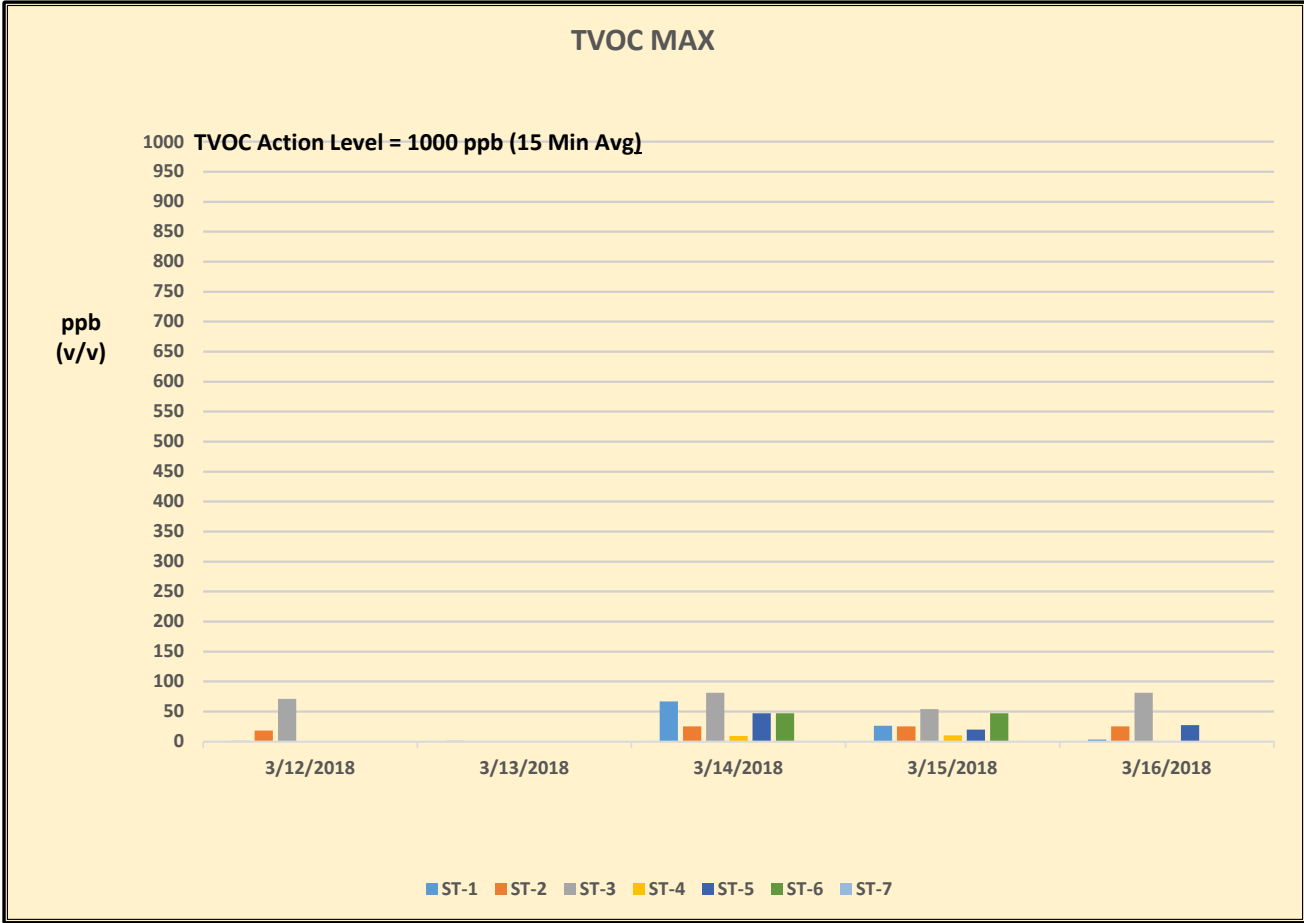
Figure 1 Gowanus Canal Superfund Site -TB4 Dredging and Capping Pilot Program TVOC Monitoring Data - Week 23
