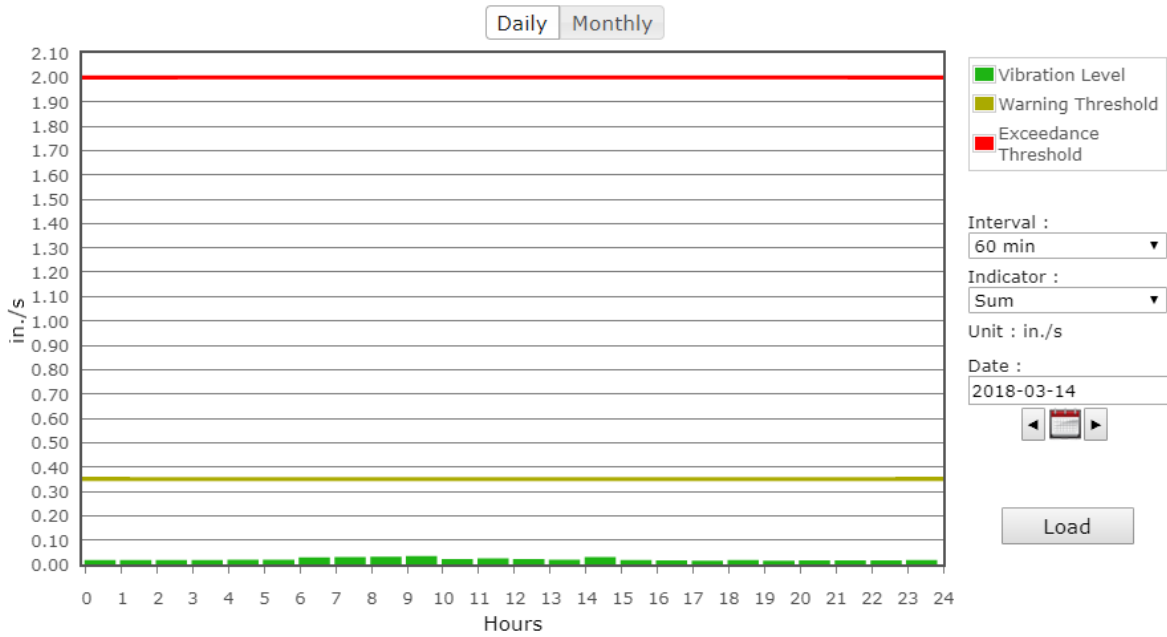
Figure 24: South Vibration Monitor VM-2 on Wednesday
