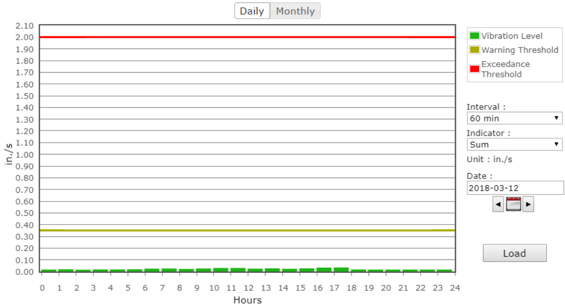
Figure 22: South Vibration Monitor VM-2 on Monday
