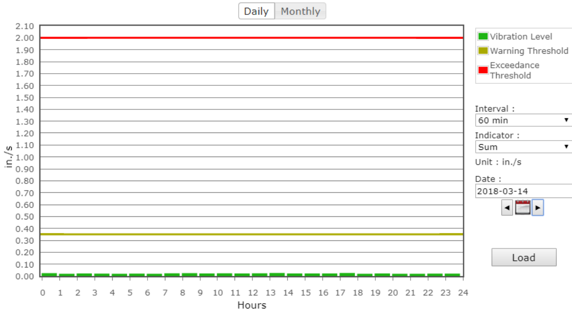
Figure 19: North Vibration Monitor VM-1 on Wednesday
