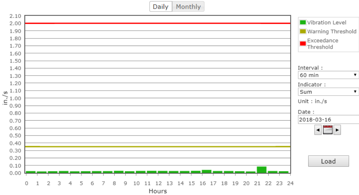
Figure 21: North Vibration Monitor VM-1 on Friday
