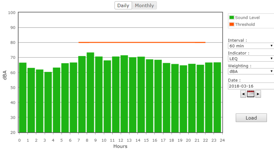
Figure 16: Northeast Monitor NM-3 on Friday
