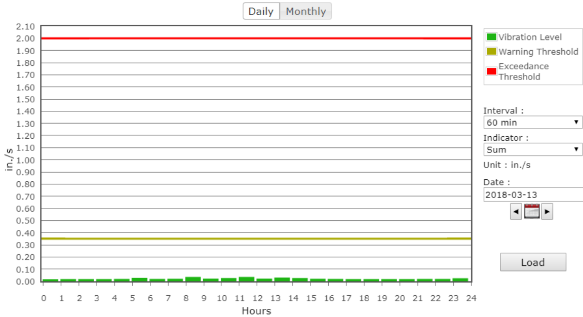
Figure 23: South Vibration Monitor VM-2 on Tuesday
