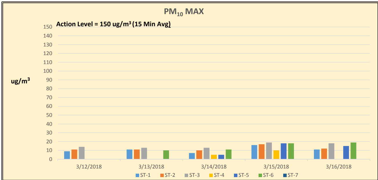
Figure 2 Gowanus Canal Superfund Site - TB4 Dredging and Capping Pilot Program TRC CAMP PM 10 Monitoring Data - Week 23
