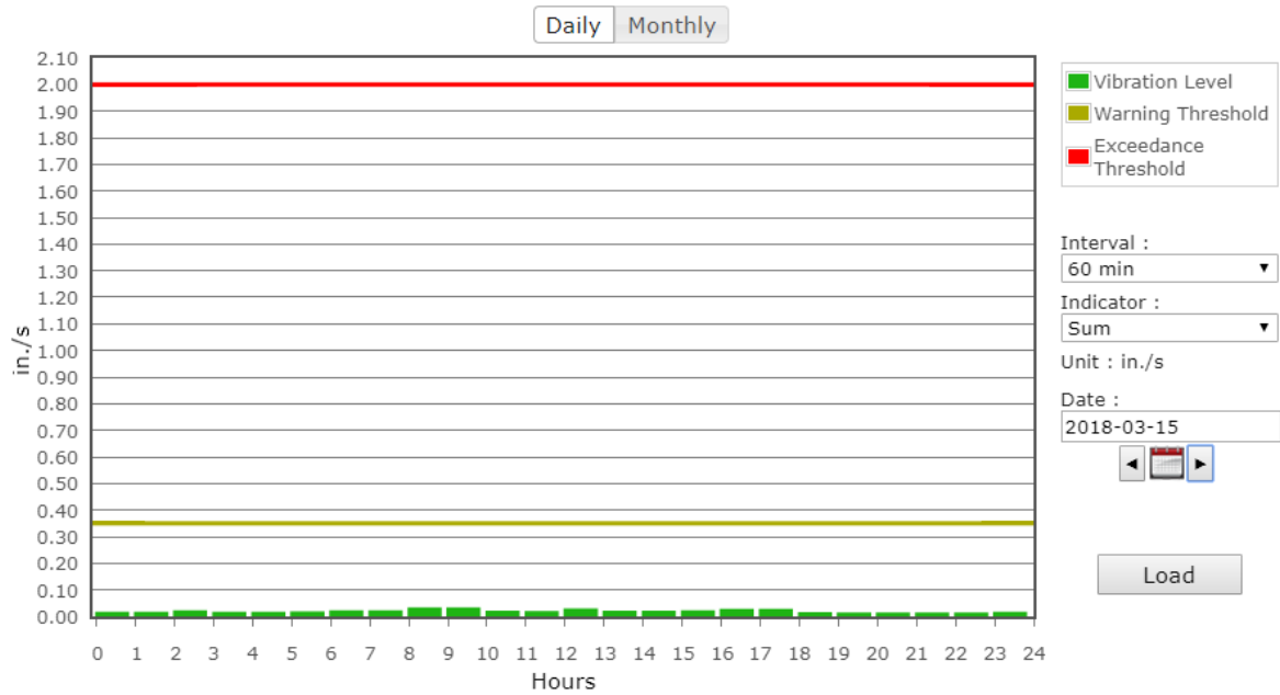
Figure 25: South Vibration Monitor VM-2 on Thursday
