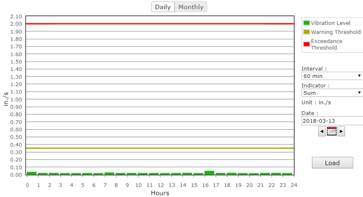
Figure 18: North Vibration Monitor VM-1 on Tuesday
