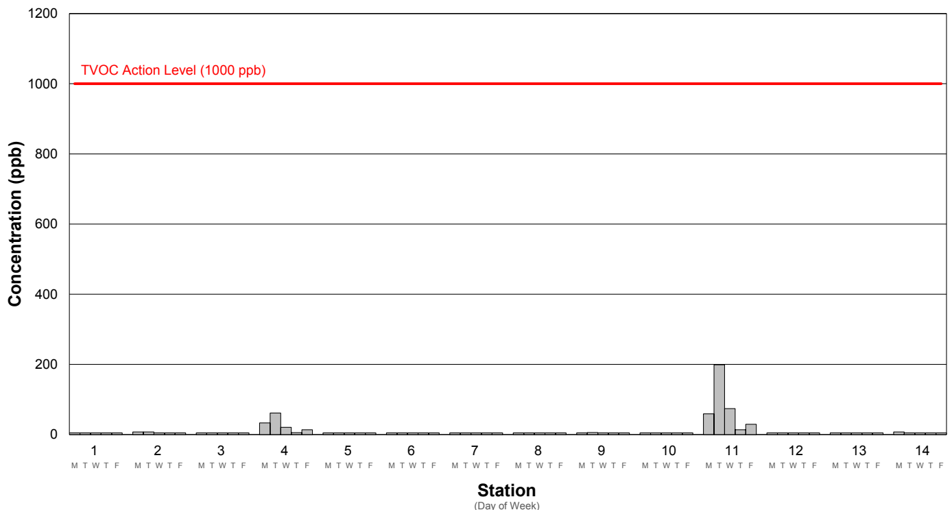
Average TVOC Concentration Week 50: 10/25/2021 - 10/29/2021
