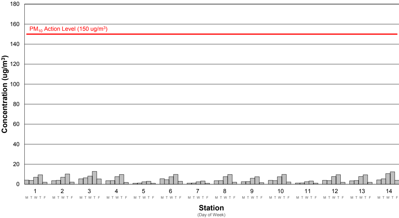
Average PM10 Concentration Week 53: 11/15/2021 - 11/19/2021
