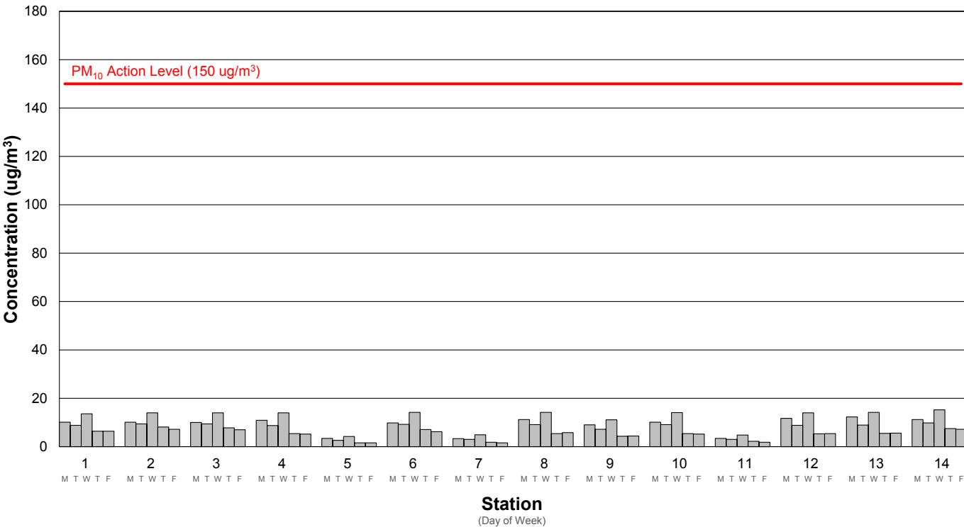
Average PM10 Concentration Week 65: 2/7/2022 - 2/11/2022
