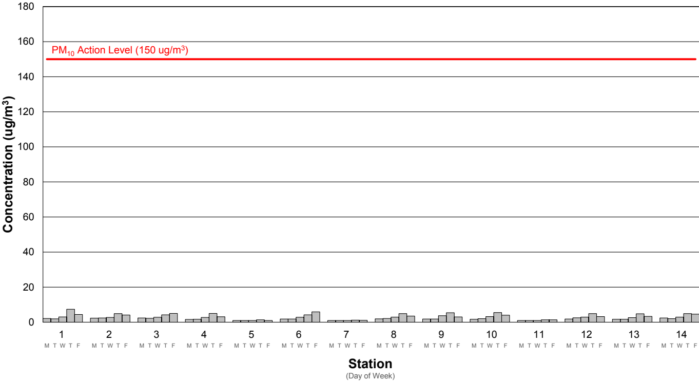
Average PM10 Concentration Week 71: 3/21/2022 - 3/25/2022
