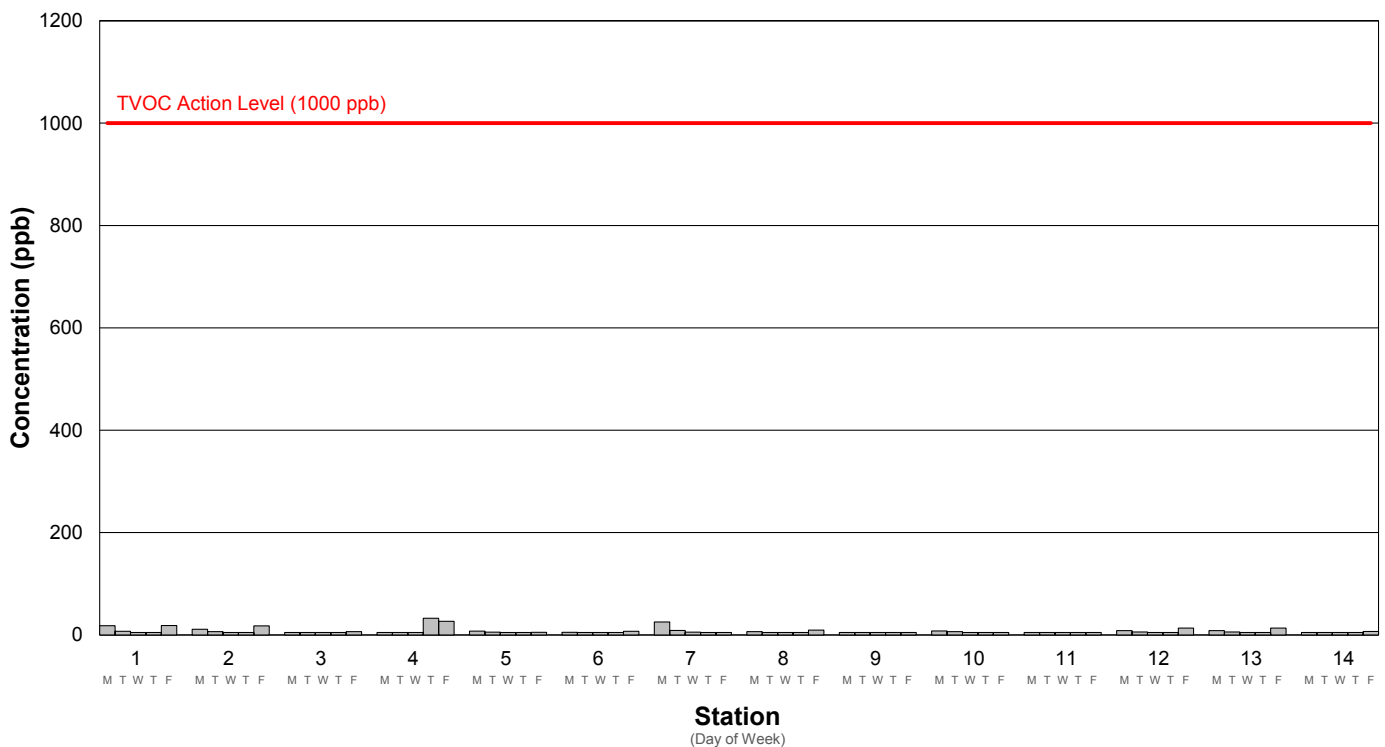
Average TVOC Concentration Week 71: 3/21/2022 - 3/25/2022
