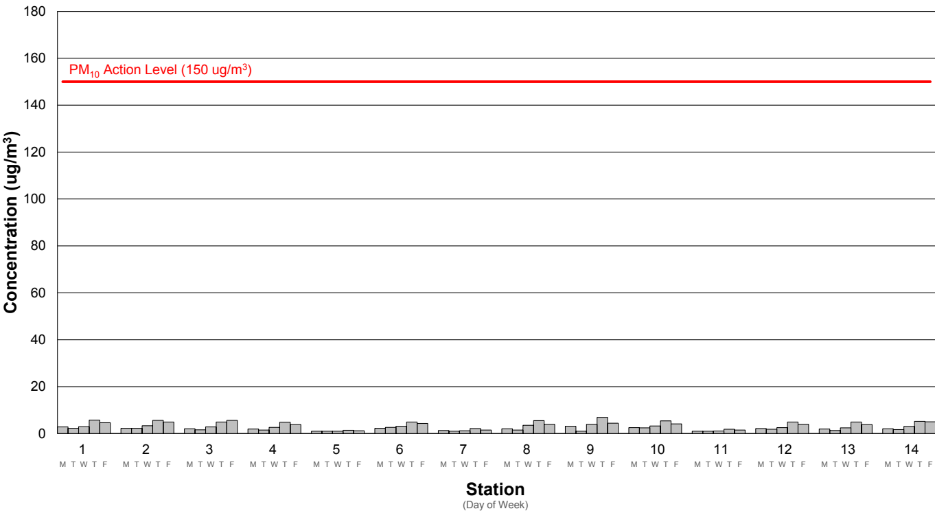
Average PM10 Concentration Week 75: 4/18/2022 - 4/22/2022
