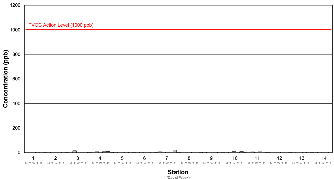
Average TVOC Concentration Week 75: 4/18/2022 - 4/22/2022
