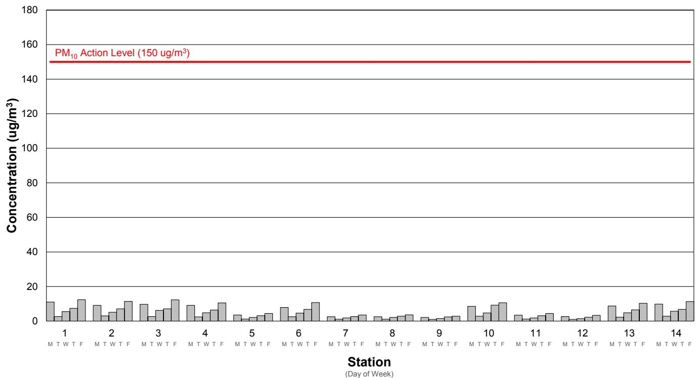
Average PM 10 Concentration Week 85: 6/27/2022 - 7/1/2022
