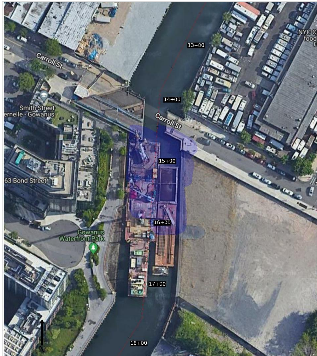
Figure 1 - Approximate areas of Phase III material dredged north of 3 RD Street Bridge between August 29 and September 1, 2022.
