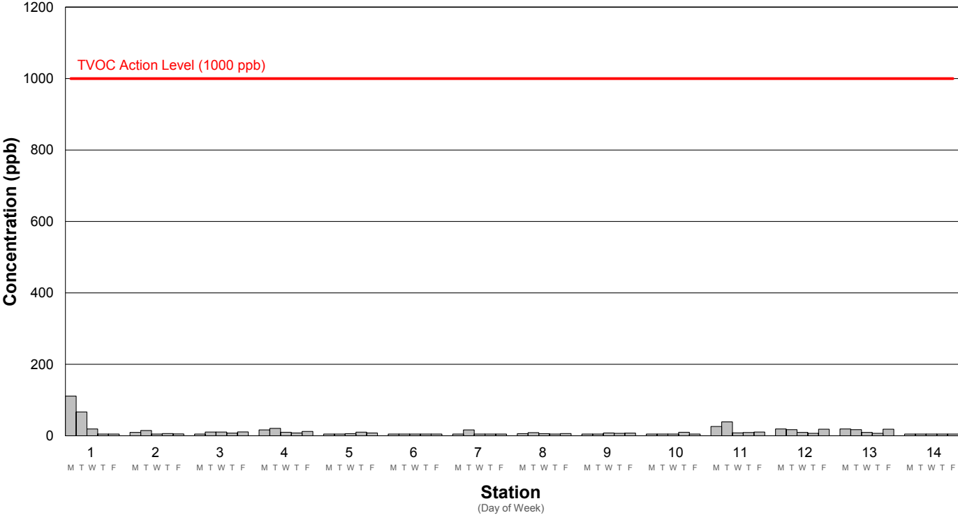
Average TVOC Concentration Week 93: 8/22/2022 - 8/26/2022
