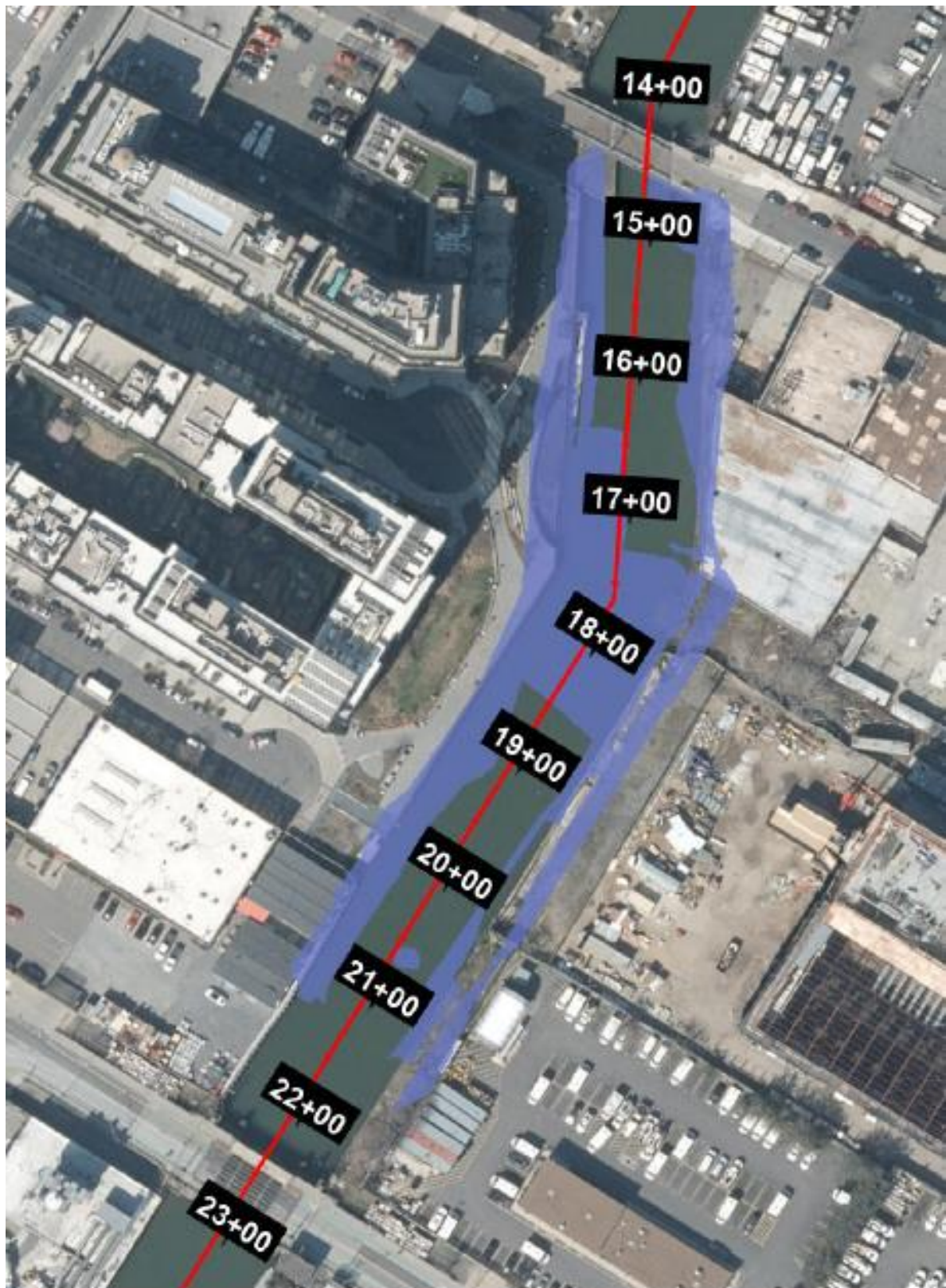
Figure 1 - Approximate areas of Phase III material dredged north of 3RD Street Bridge between September 9 and September 22, 2022.
