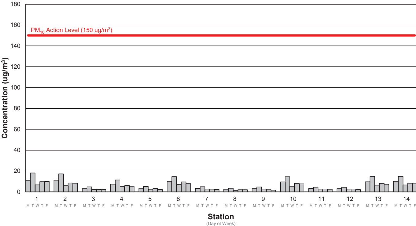
Average PM10 Concentration Week 113: 1/9/2023 - 1/13/2023
