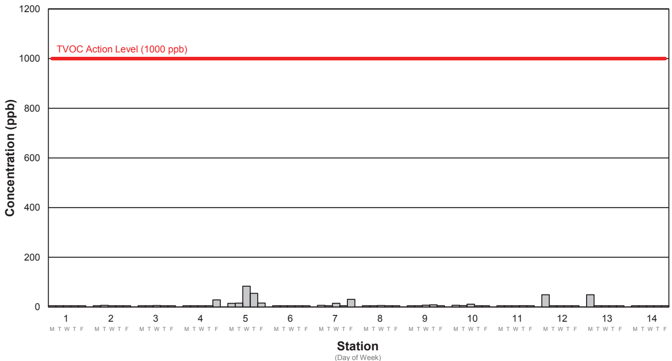
Average TVOC Concentration Week 110: 12/19/2022 - 12/23/2022
