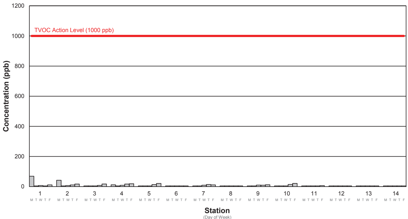
Average TVOC Concentration Week 111: 12/26/2022 - 12/30/2022
