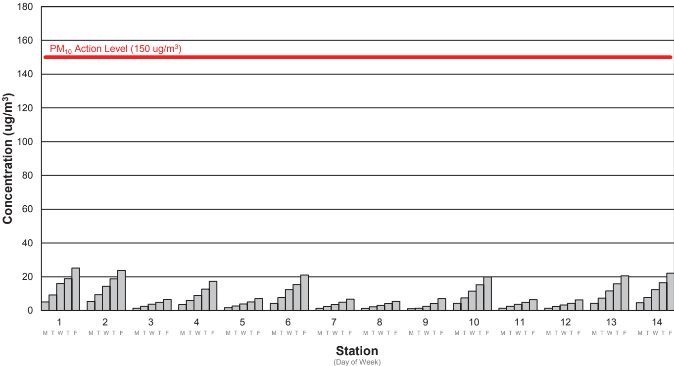
Average PM10 Concentration Week 111: 12/26/2022 - 12/30/2022
