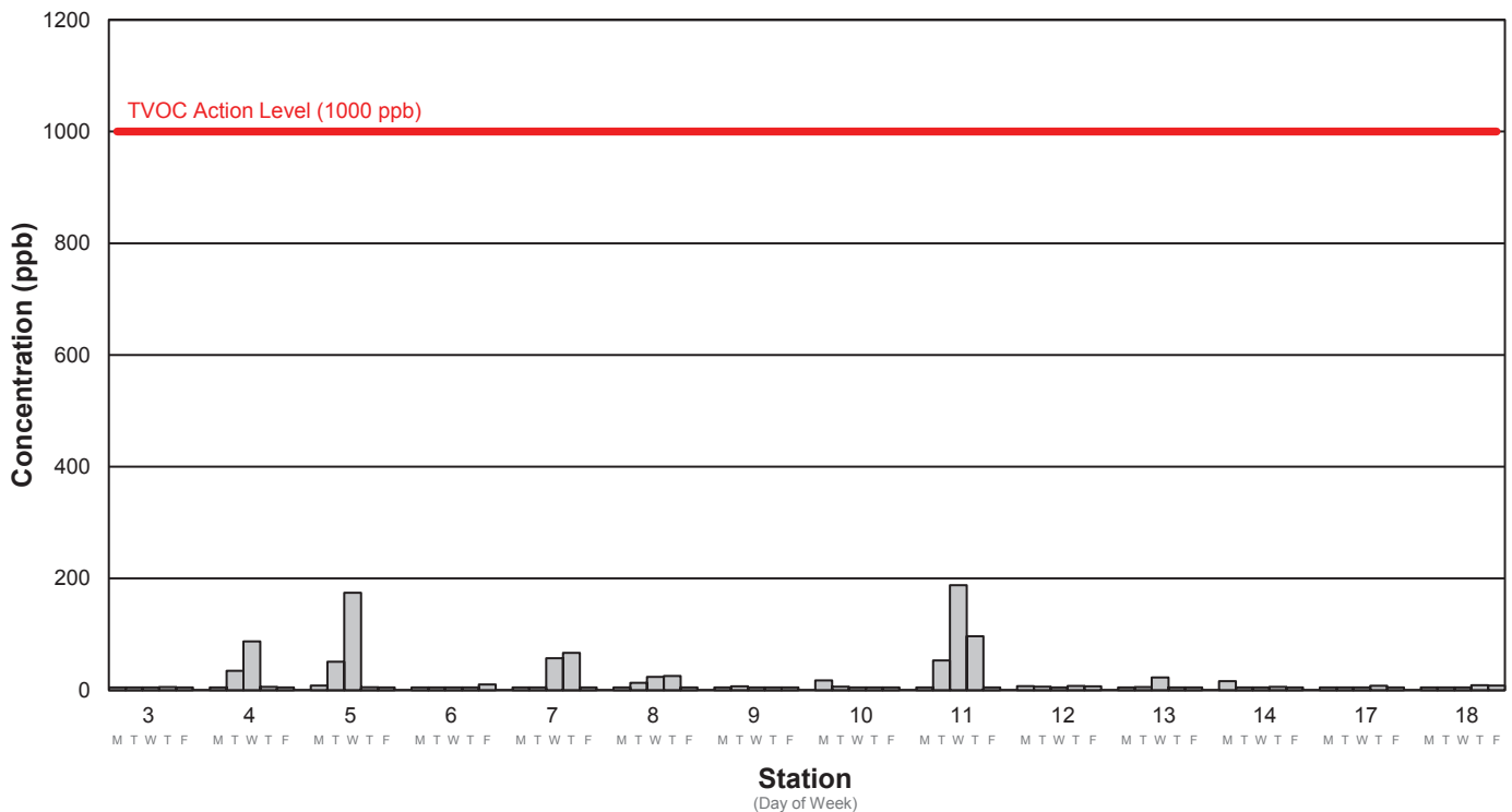
Average TVOC Concentration Week 125: 4/3/2023 - 4/7/2023
