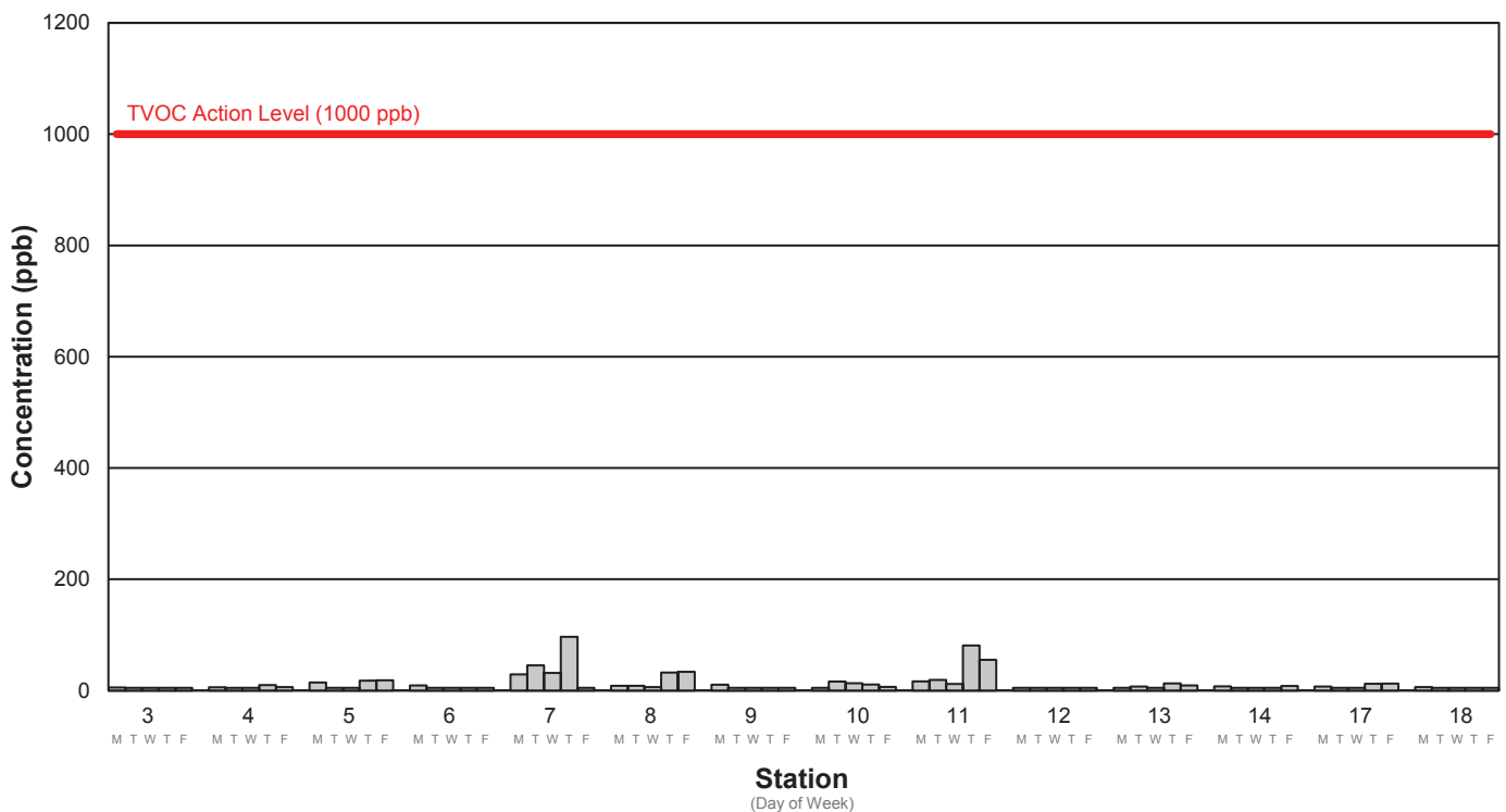
Average TVOC Concentration Week 129: 5/1/2023 - 5/5/2023
