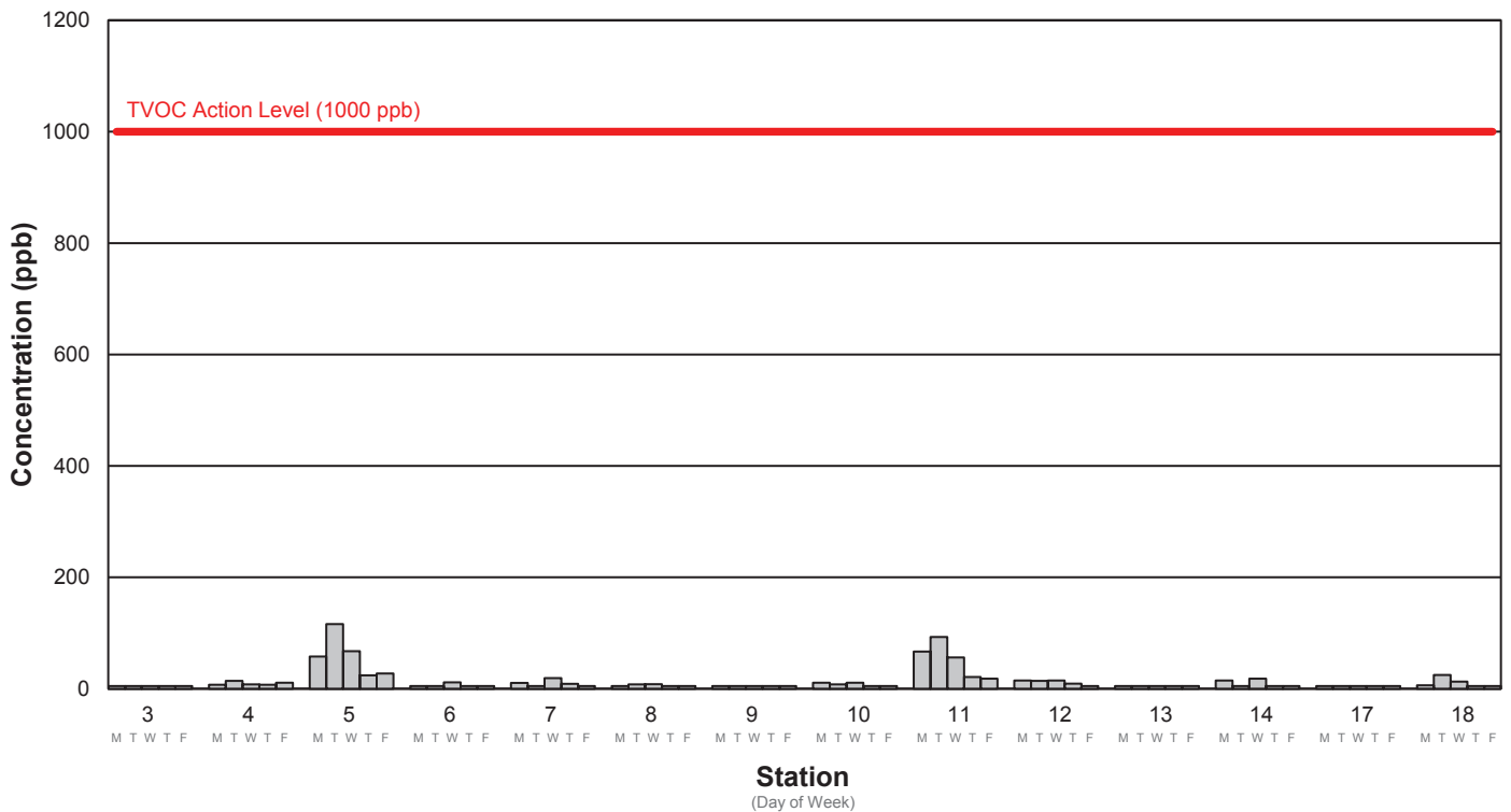
Average TVOC Concentration Week 138: 7/3/2023 - 7/7/2023
