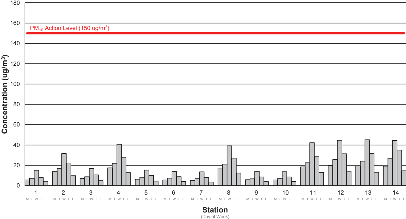
Average PM10 Concentration Week 140: 7/17/2023 - 7/21/2023
