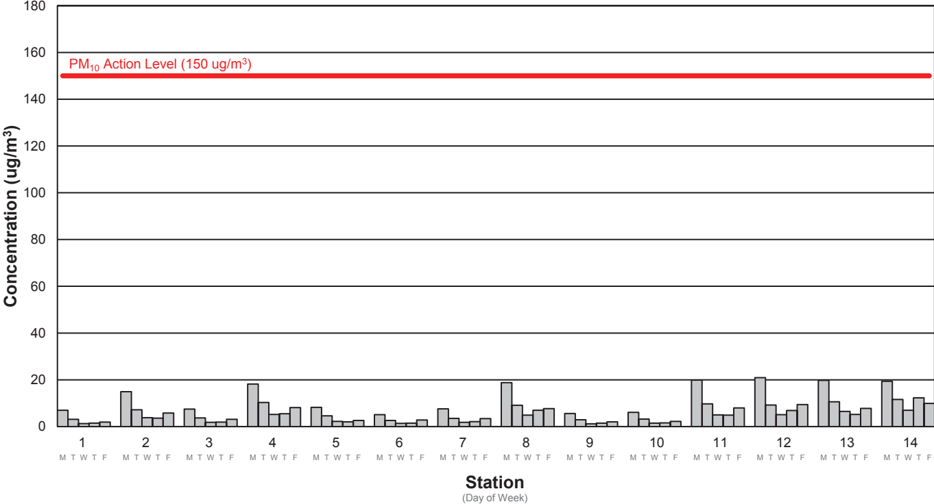
Average PM10 Concentration Week 145: 8/21/2023 - 8/25/2023
