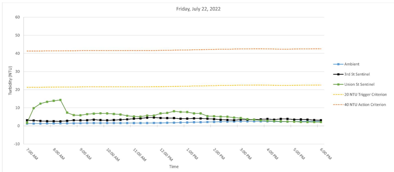
Figure 6. Hourly rolling average turbidity readings on Friday, July 22, 2022, from 7 AM to 6 PM.
