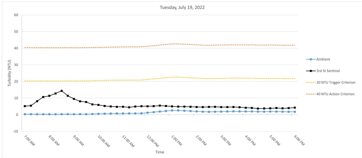
Figure 3. Hourly rolling average turbidity readings on Tuesday, July 19, 2022, from 7 AM to 6 PM.
