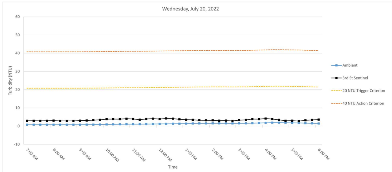
Figure 4. Hourly rolling average turbidity readings on Wednesday, July 20, 2022, from 7 AM to 6 PM.
