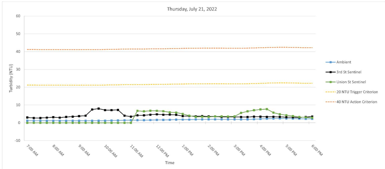
Figure 5. Hourly rolling average turbidity readings on Thursday, July 21, 2022, from 7 AM to 6 PM.
