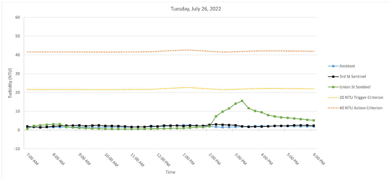
Figure 3. Hourly rolling average turbidity readings on Tuesday, July 26, 2022, from 7 AM to 6 PM.
