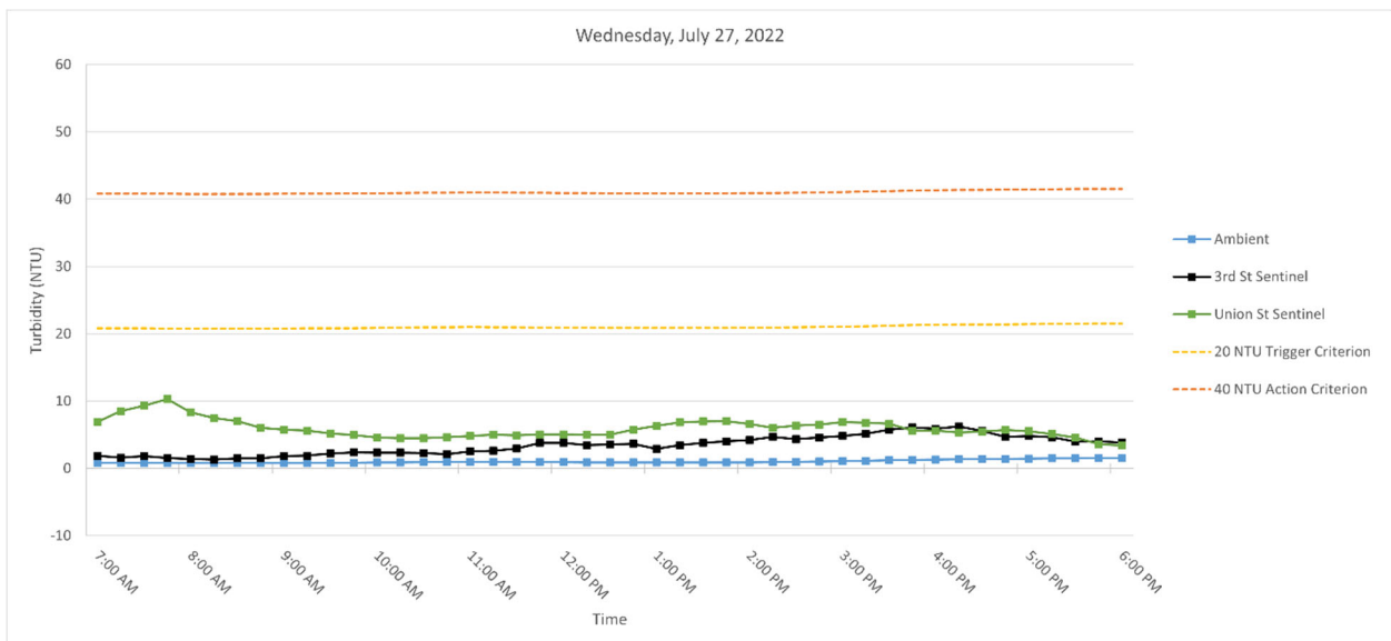
Figure 4. Hourly rolling average turbidity readings on Wednesday, July 27, 2022, from 7 AM to 6 PM.
