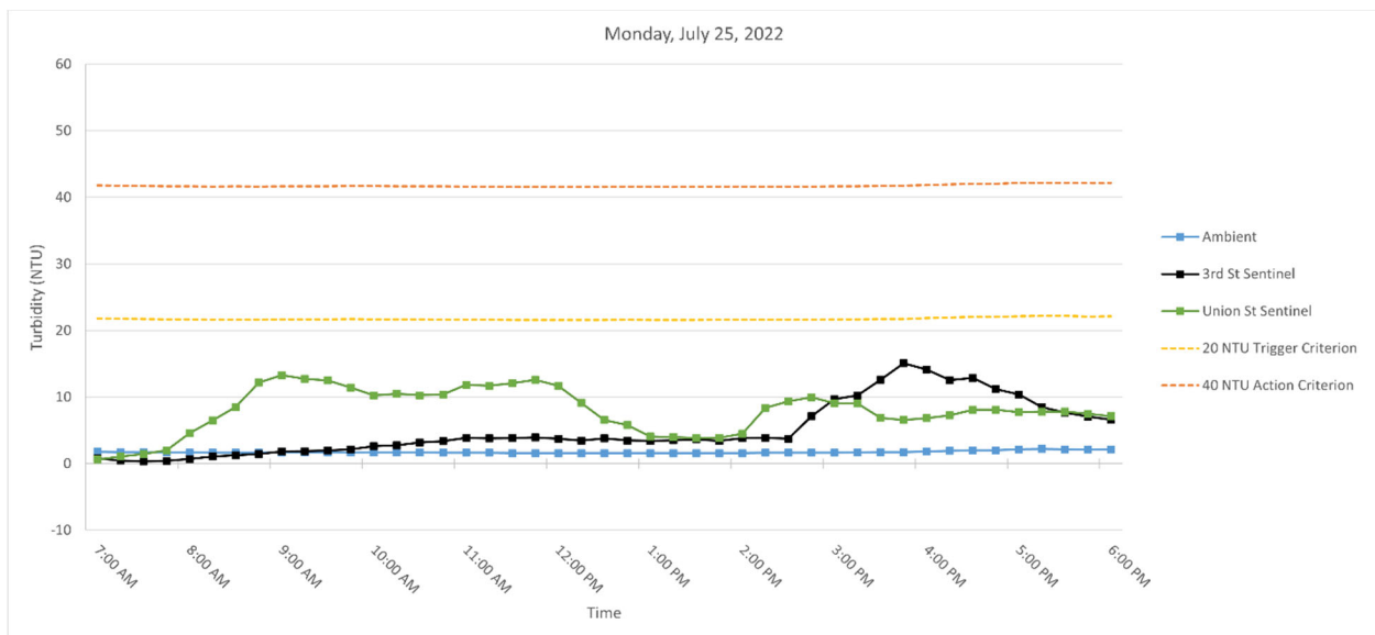
Figure 2. Hourly rolling average turbidity readings on Monday, July 25, 2022, from 7 AM to 6 PM.
