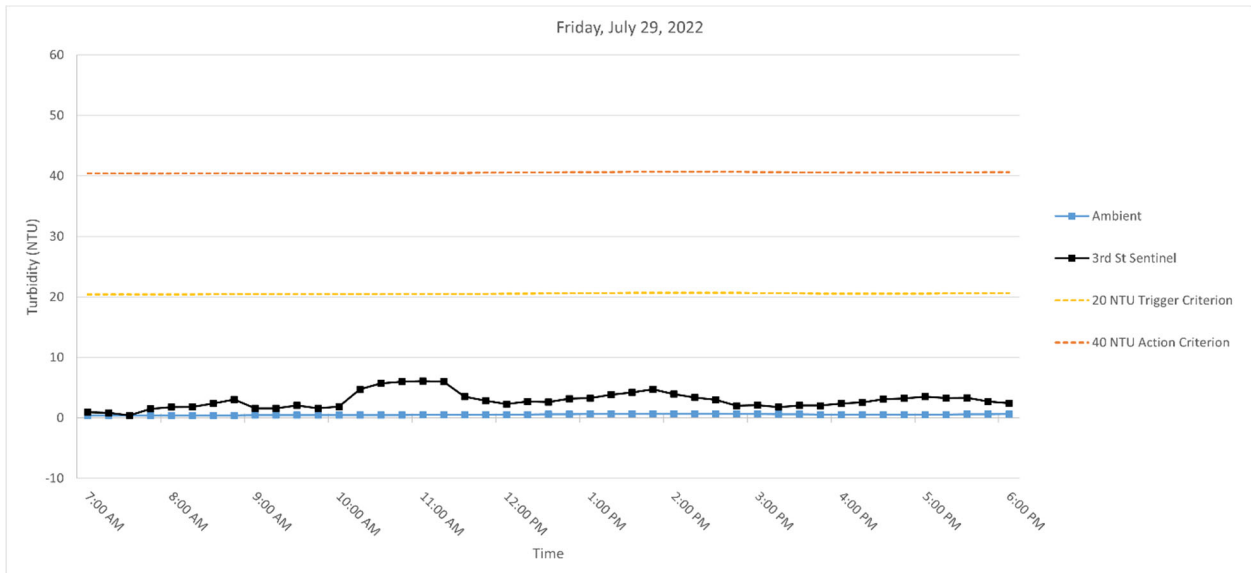
Figure 6. Hourly rolling average turbidity readings on Friday, July 29, 2022, from 7 AM to 6 PM.
