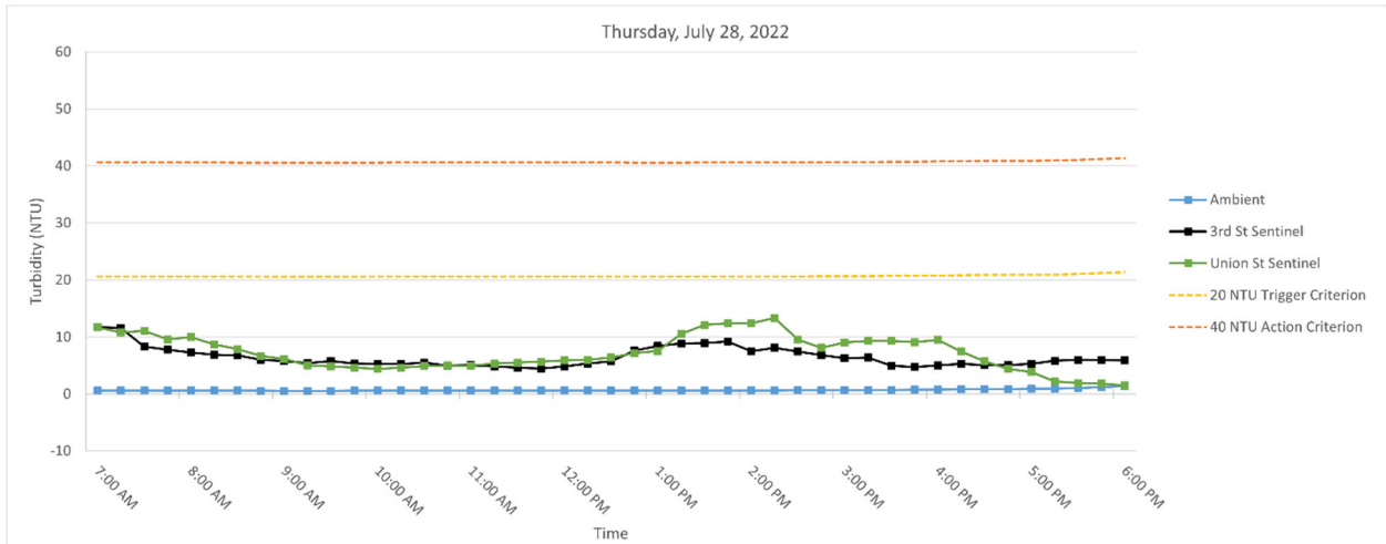
Figure 5. Hourly rolling average turbidity readings on Thursday, July 28, 2022, from 7 AM to 6 PM.
