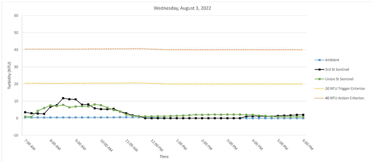
Figure 4. Hourly rolling average turbidity readings on Wednesday, August 3, 2022, from 7 AM to 6 PM.
