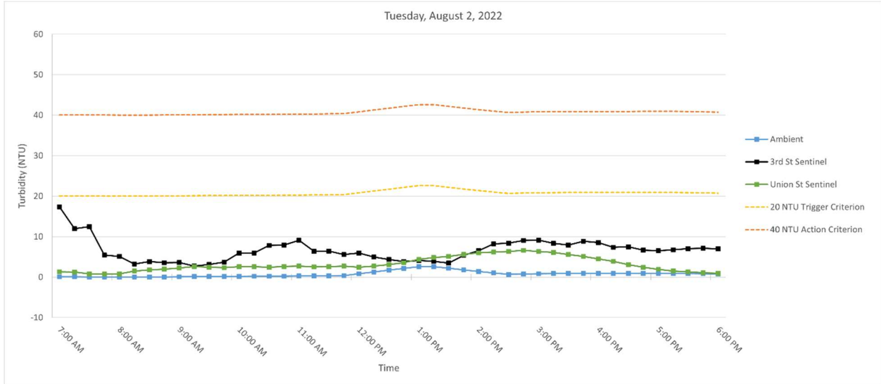
Figure 3. Hourly rolling average turbidity readings on Tuesday, August 2, 2022, from 7 AM to 6 PM.
