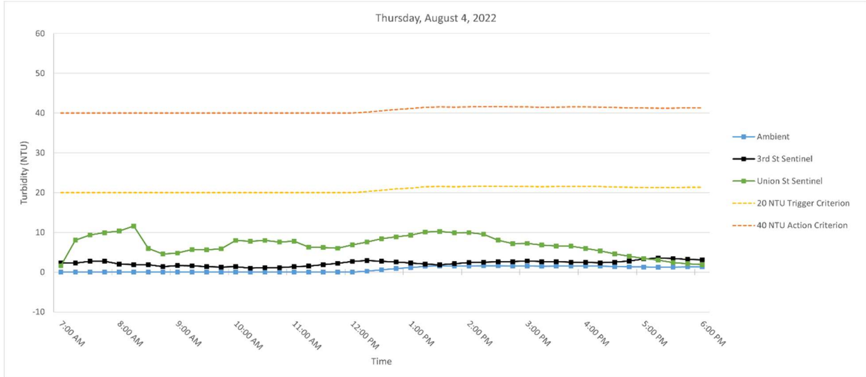
Figure 5. Hourly rolling average turbidity readings on Thursday, August 4, 2022, from 7 AM to 6 PM.
