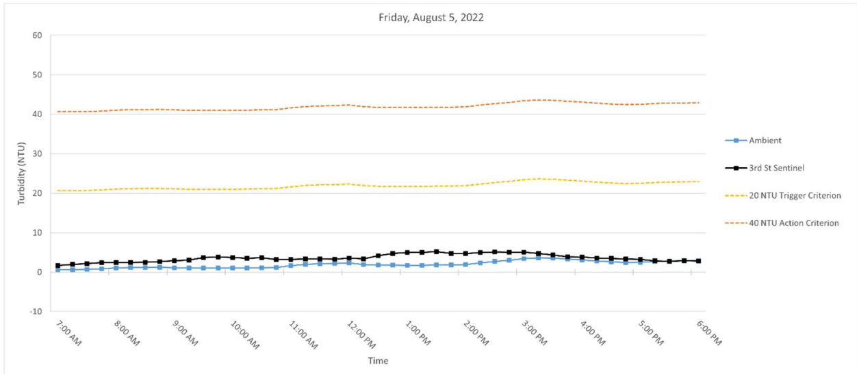
Figure 6. Hourly rolling average turbidity readings on Friday, August 5, 2022, from 7 AM to 6 PM.
