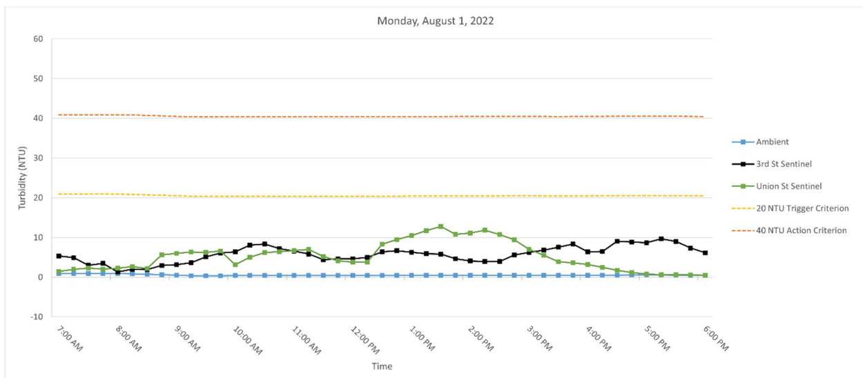
Figure 2. Hourly rolling average turbidity readings on Monday, August 1, 2022, from 7 AM to 6 PM.
