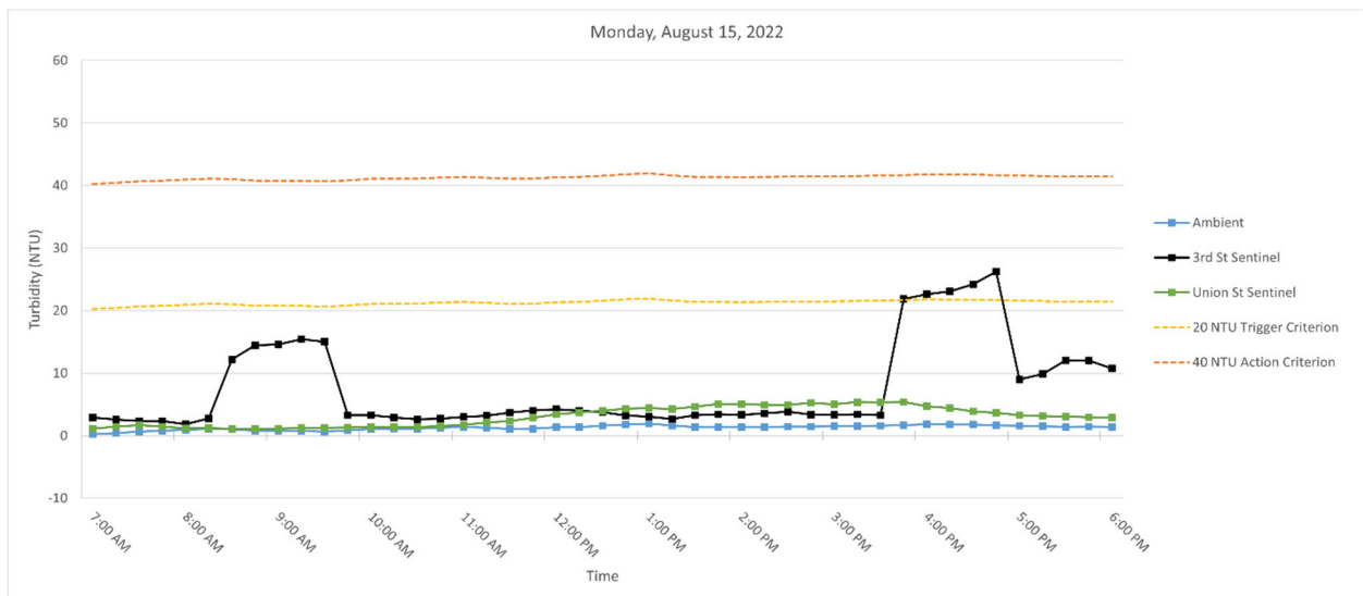
Figure 2. Hourly rolling average turbidity readings on Monday, August 15, 2022, from 7 AM to 6 PM.
