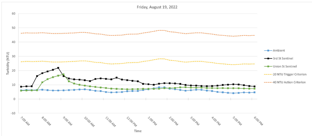
Figure 6. Hourly rolling average turbidity readings on Friday, August 19, 2022, from 7 AM to 6 PM.
