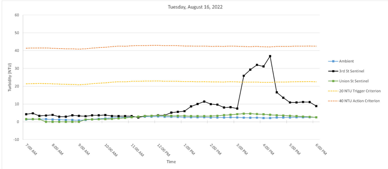
Figure 3. Hourly rolling average turbidity readings on Tuesday, August 16, 2022, from 7 AM to 6 PM.
