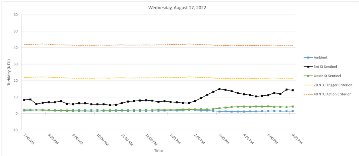
Figure 4. Hourly rolling average turbidity readings on Wednesday, August 17, 2022, from 7 AM to 6 PM.
