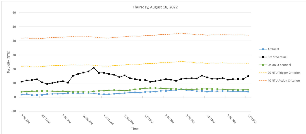
Figure 5. Hourly rolling average turbidity readings on Thursday, August 18, 2022, from 7 AM to 6 PM.
