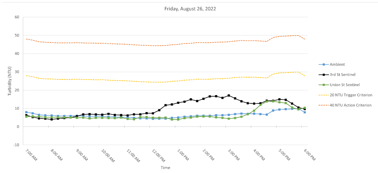
Figure 6. Hourly rolling average turbidity readings on Friday, August 26, 2022, from 7 AM to 6 PM.
