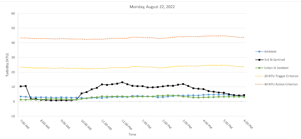
Figure 2. Hourly rolling average turbidity readings on Monday, August 22, 2022, from 7 AM to 6 PM.
