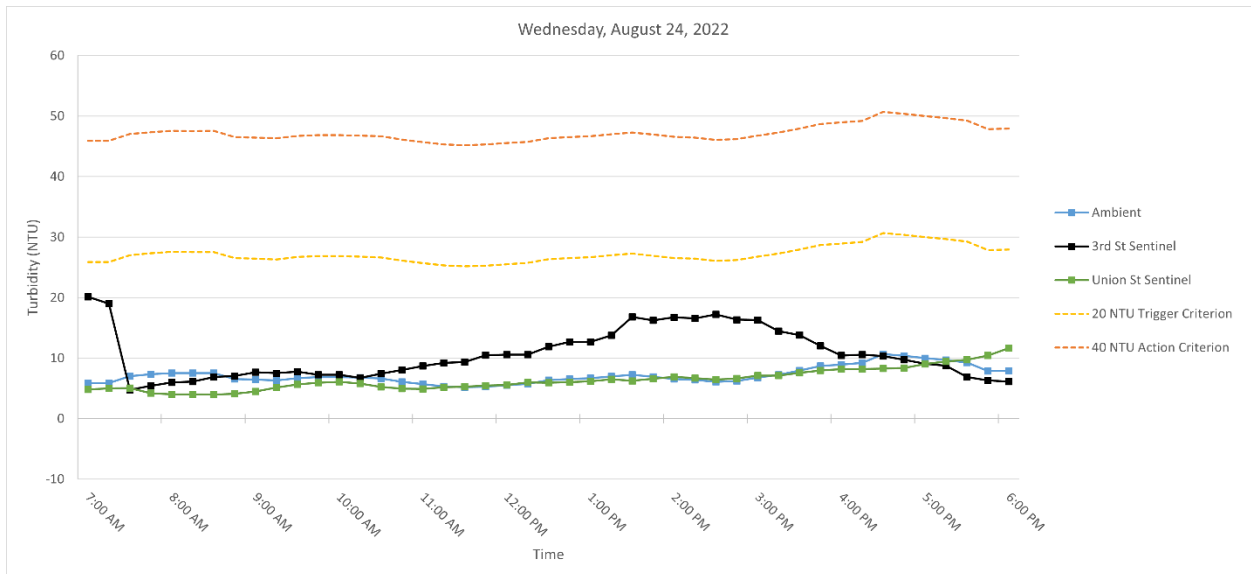
Figure 4. Hourly rolling average turbidity readings on Wednesday, August 24, 2022, from 7 AM to 6 PM.
