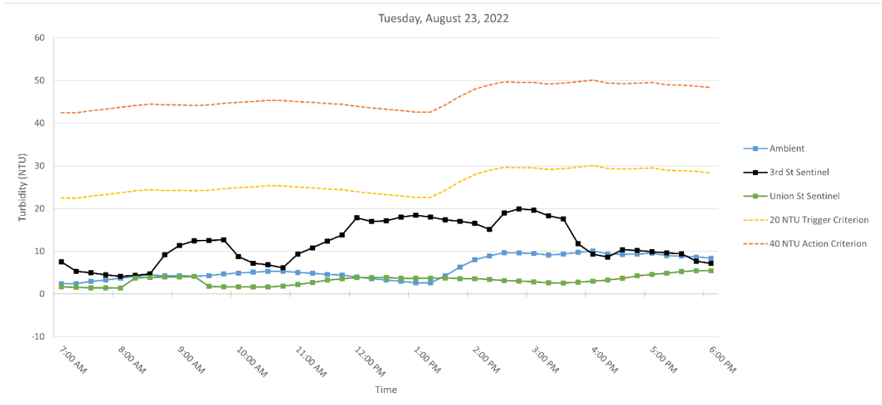
Figure 3. Hourly rolling average turbidity readings on Tuesday, August 23, 2022, from 7 AM to 6 PM.
