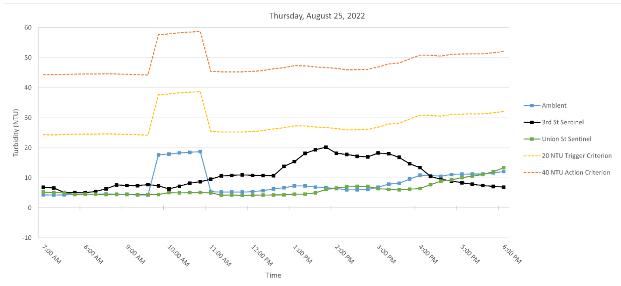
Figure 5. Hourly rolling average turbidity readings on Thursday, August 25, 2022, from 7 AM to 6 PM.
