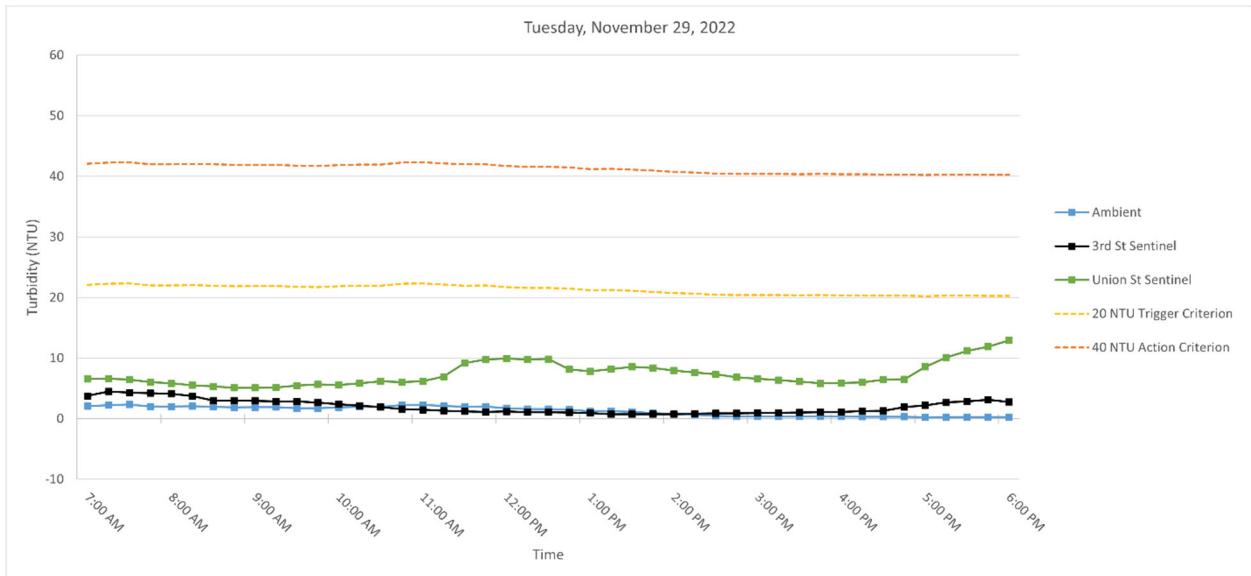
Figure 3. Hourly rolling average turbidity readings on Tuesday, November 29, 2022, from 7 AM to 6 PM.
