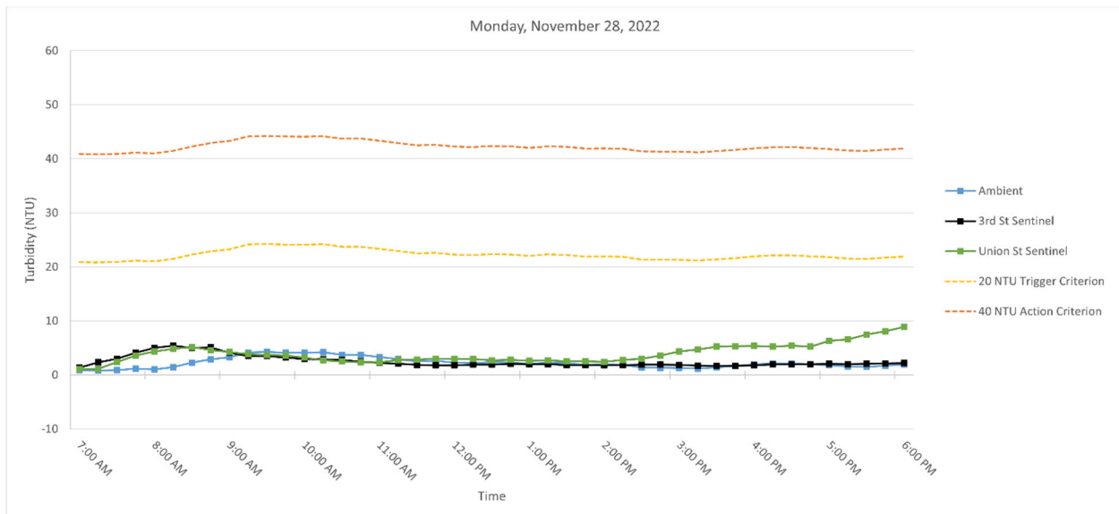
Figure 3. Hourly rolling average turbidity readings on Monday, November 28, 2022, from 7 AM to 6 PM.
