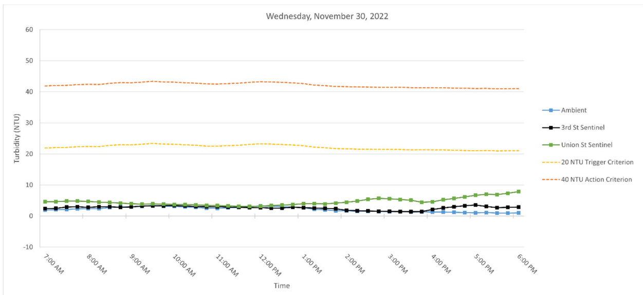
Figure 4. Hourly rolling average turbidity readings on Wednesday, November 30, 2022, from 7 AM to 6 PM.
