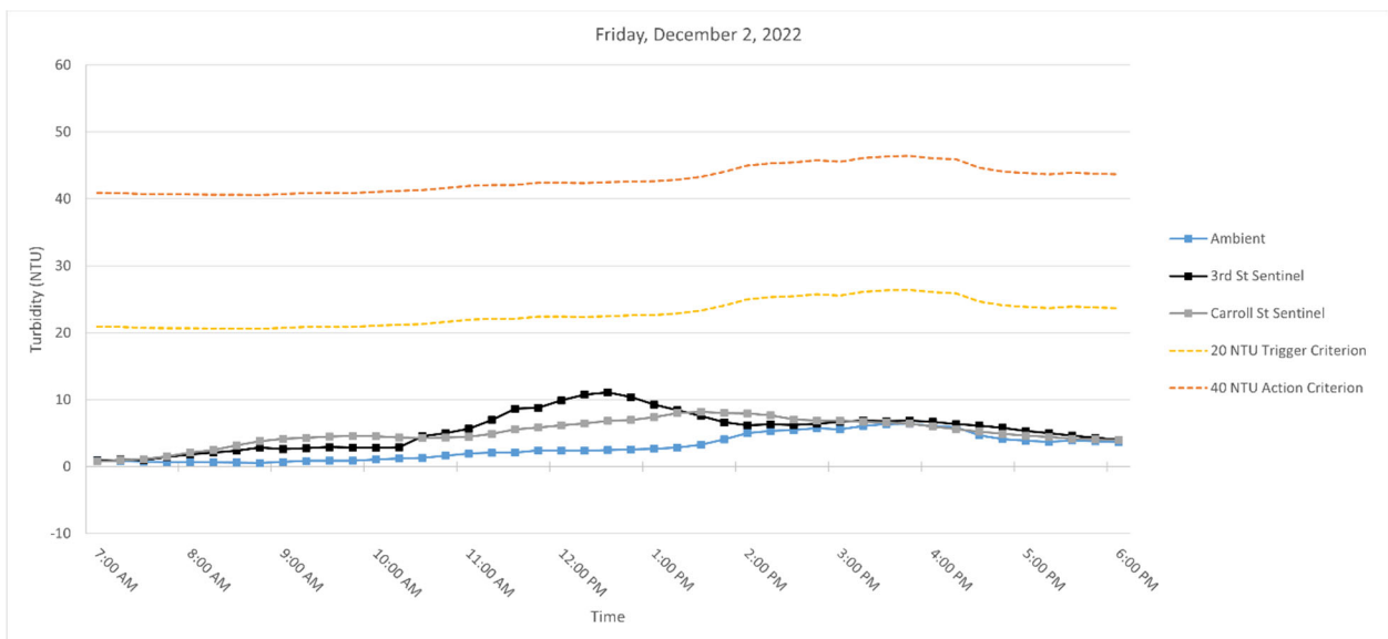
Figure 6. Hourly rolling average turbidity readings on Friday, December 2, 2022, from 7 AM to 6 PM.
