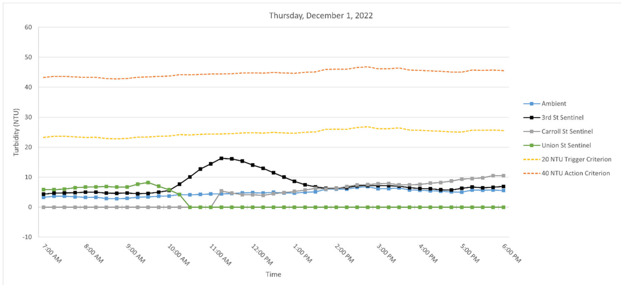
Figure 5. Hourly rolling average turbidity readings on Thursday, December 1, 2022, from 7 AM to 6 PM.
