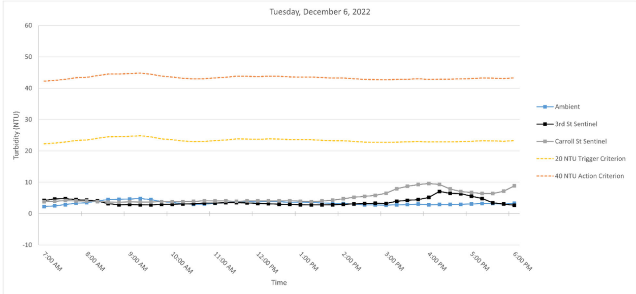
Figure 3. Hourly rolling average turbidity readings on Tuesday, December 6, 2022, from 7 AM to 6 PM.
