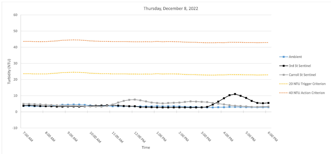
Figure 5. Hourly rolling average turbidity readings on Thursday, December 8, 2022, from 7 AM to 6 PM.
