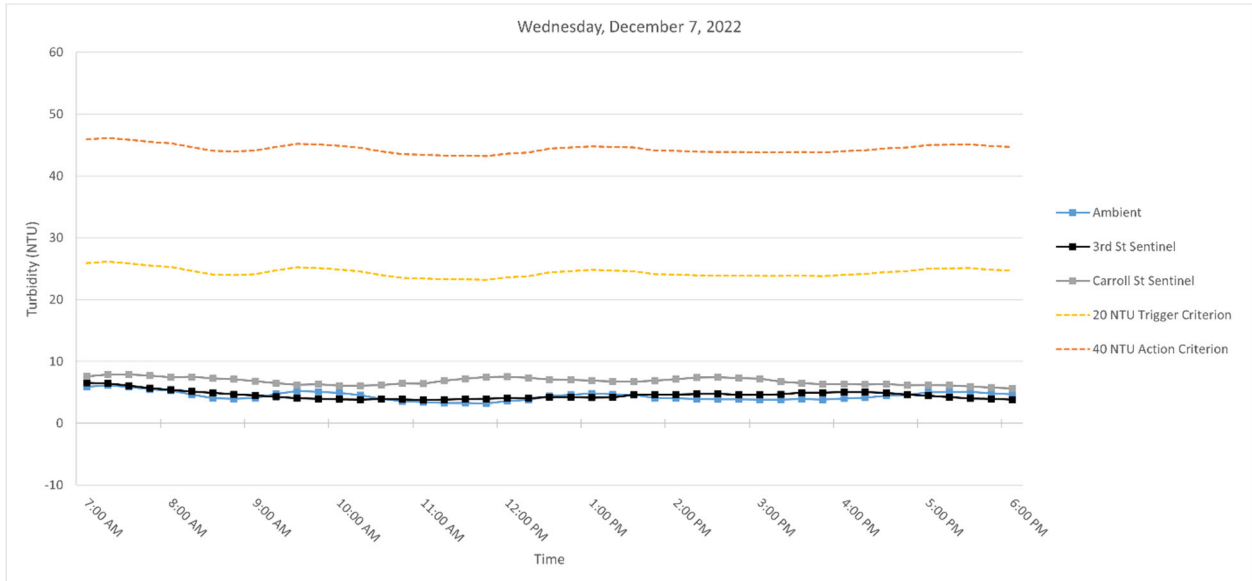
Figure 4. Hourly rolling average turbidity readings on Wednesday, December 7, 2022, from 7 AM to 6 PM.
