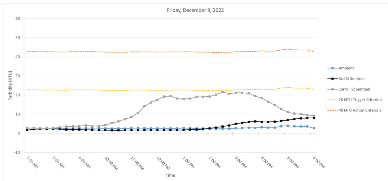
Figure 6. Hourly rolling average turbidity readings on Friday, December 9, 2022, from 7 AM to 6 PM.
