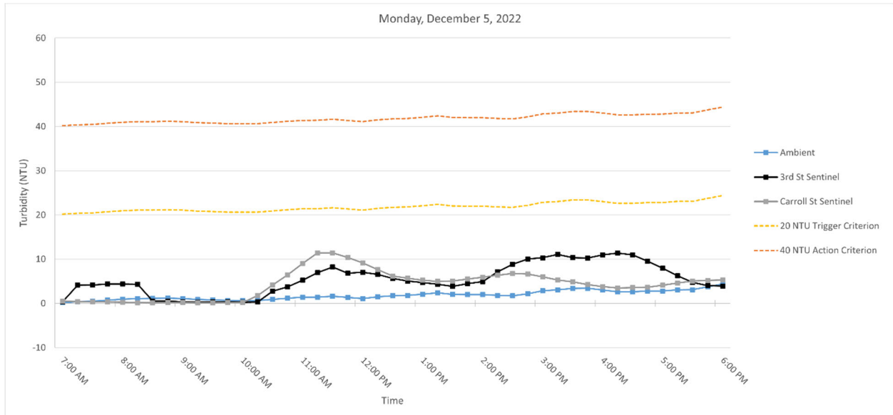
Figure 3. Hourly rolling average turbidity readings on Monday, December 5, 2022, from 7 AM to 6 PM.
