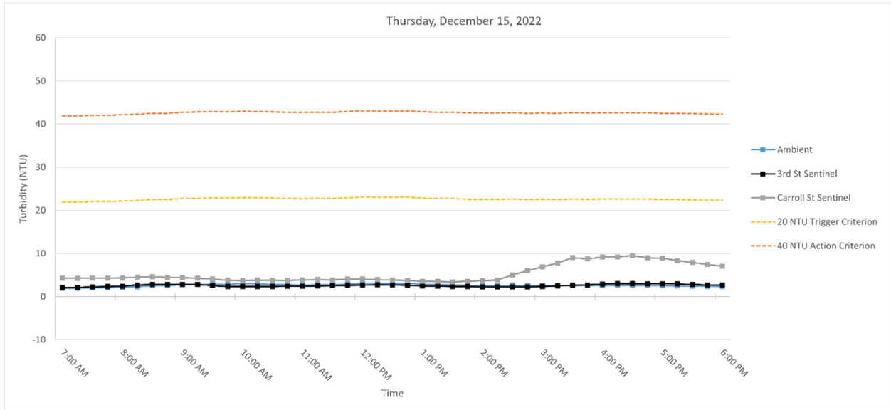
Figure 5. Hourly rolling average turbidity readings on Thursday, December 15, 2022, from 7 AM to 6 PM.
