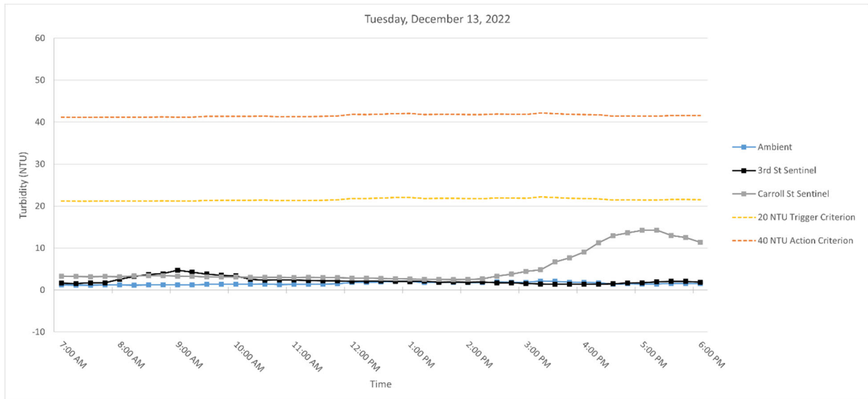
Figure 3. Hourly rolling average turbidity readings on Tuesday, December 13, 2022, from 7 AM to 6 PM.
