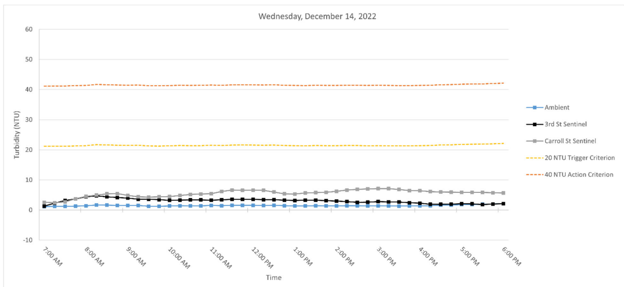
Figure 4. Hourly rolling average turbidity readings on Wednesday, December 14, 2022, from 7 AM to 6 PM.
