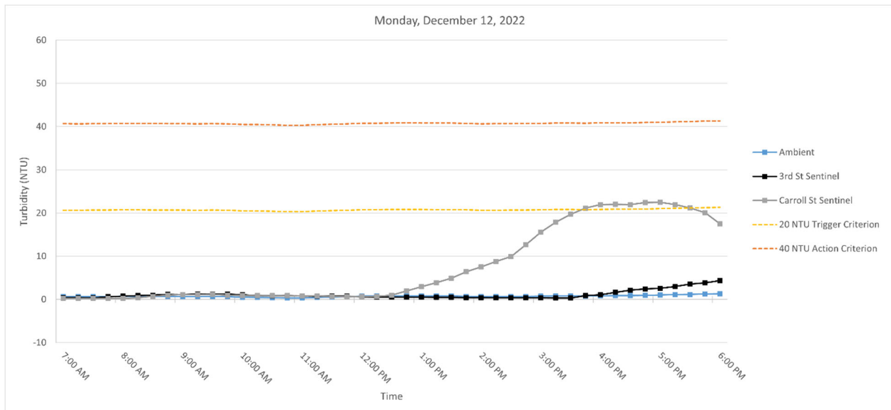
Figure 3. Hourly rolling average turbidity readings on Monday, December 12, 2022, from 7 AM to 6 PM.
