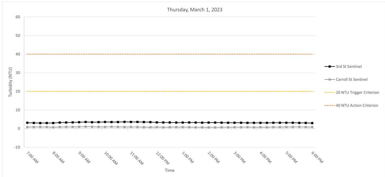
Figure 5. Hourly rolling average turbidity readings on Thursday, March 2, 2023, from 7 AM to 6 PM.
