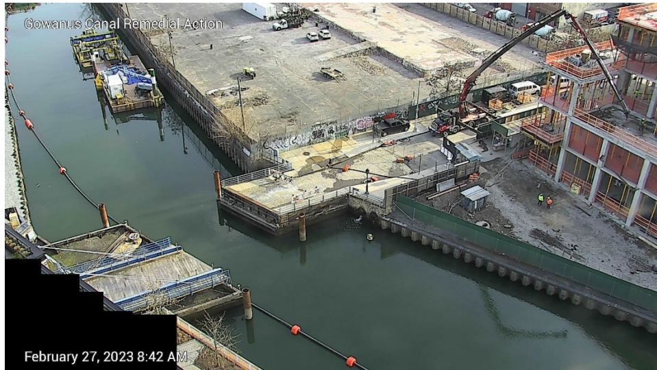
Figure 7. Discharge from high level storm sewer pipe on February 27, 2023 at 8:45 AM.
