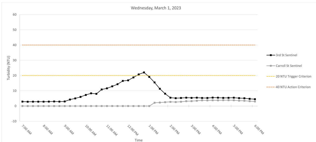
Figure 4. Hourly rolling average turbidity readings on Wednesday, March 1, 2023, from 7 AM to 6 PM.
