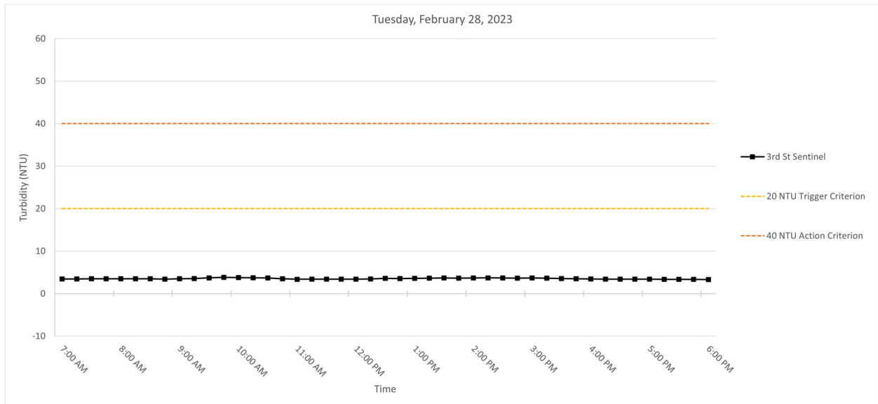
Figure 3. Hourly rolling average turbidity readings on Tuesday, February 28, 2023, from 7 AM to 6 PM.
