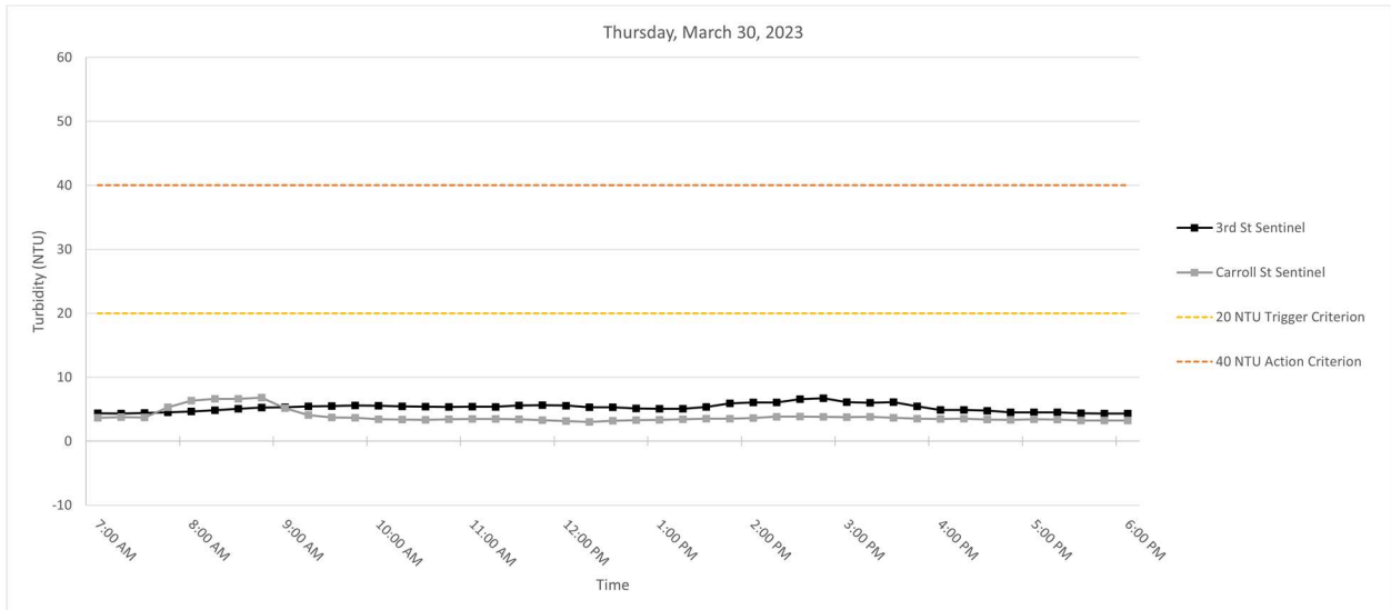
Figure 5. Hourly rolling average turbidity readings on Thursday, March 30, 2023, from 7 AM to 6 PM.
