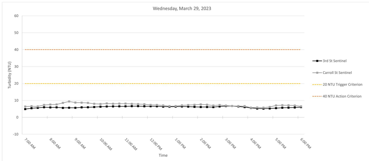
Figure 4. Hourly rolling average turbidity readings on Wednesday, March 29, 2023, from 7 AM to 6 PM.
