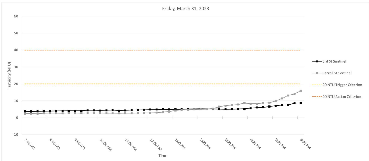
Figure 6. Hourly rolling average turbidity readings on Friday, March 31, 2023, from 7 AM to 6 PM.
