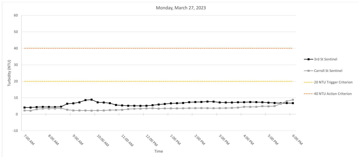
Figure 3. Hourly rolling average turbidity readings on Monday, March 27, 2023, from 7 AM to 6 PM.
