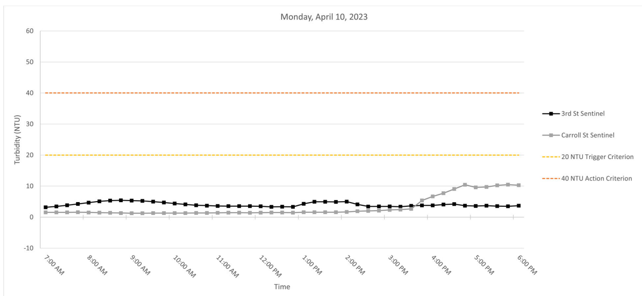
Figure 3. Hourly rolling average turbidity readings on Monday, April 10, 2023, from 7 AM to 6 PM.
