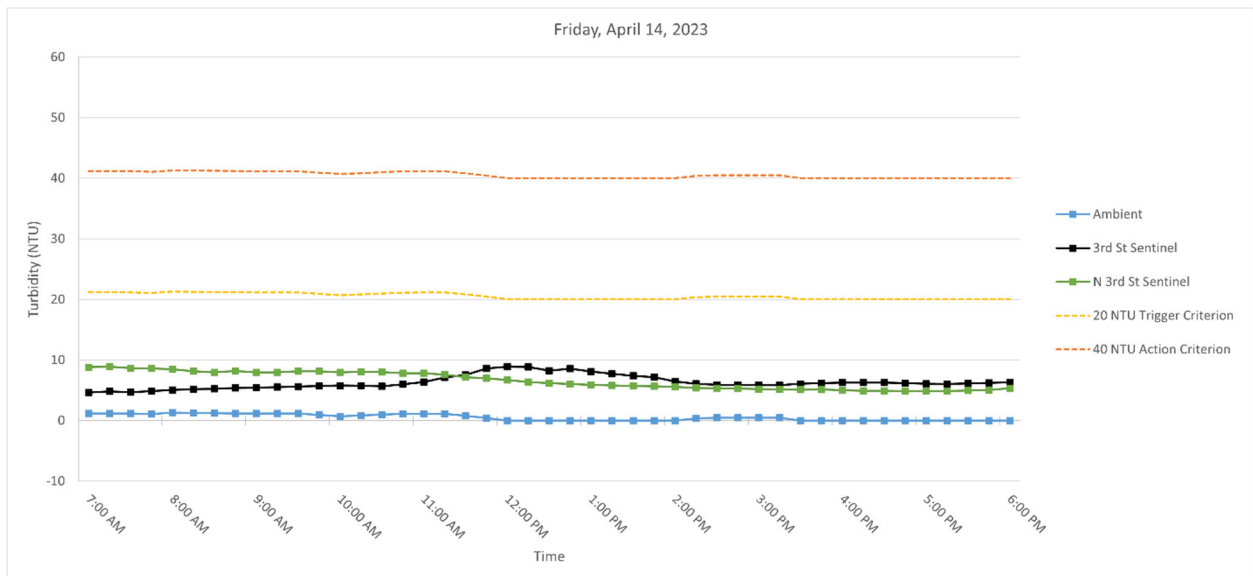
Figure 6. Hourly rolling average turbidity readings on Friday, April 14, 2023, from 7 AM to 6 PM.
