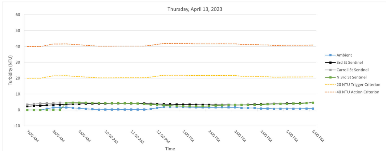
Figure 5. Hourly rolling average turbidity readings on Thursday, April 13, 2023, from 7 AM to 6 PM.
