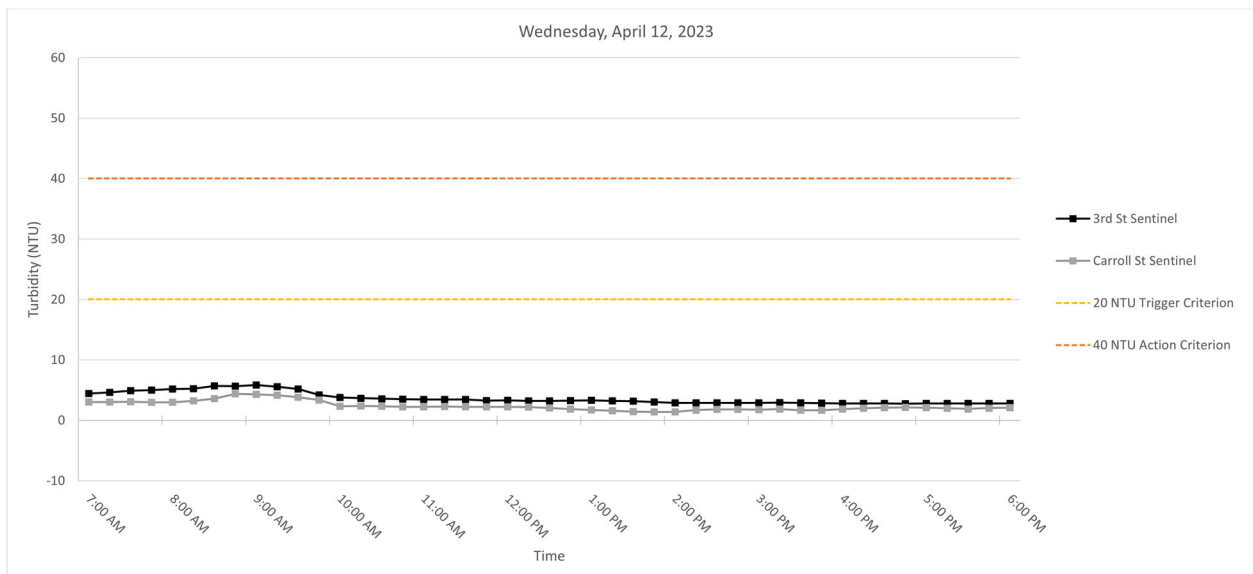
Figure 4. Hourly rolling average turbidity readings on Wednesday, April 12, 2023, from 7 AM to 6 PM.
