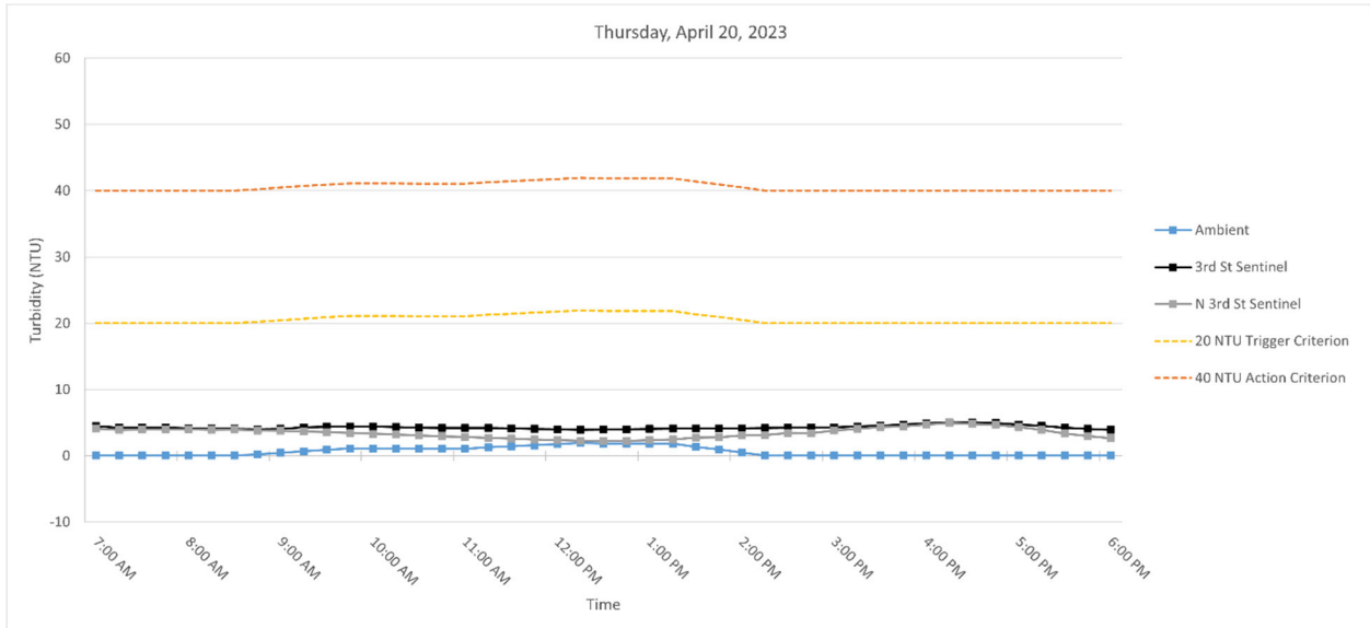
Figure 5. Hourly rolling average turbidity readings on Thursday, April 20, 2023, from 7 AM to 6 PM.
