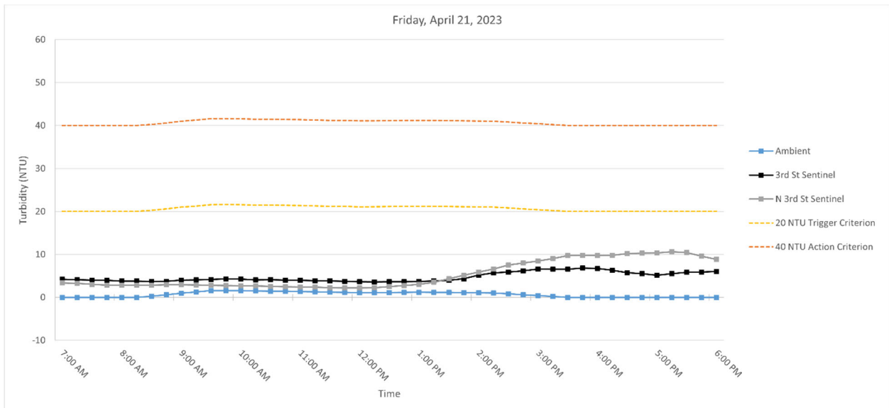
Figure 6. Hourly rolling average turbidity readings on Friday, April 21, 2023, from 7 AM to 6 PM.
