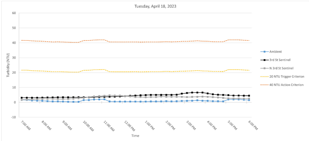
Figure 3. Hourly rolling average turbidity readings on Tuesday, April 18, 2023, from 7 AM to 6 PM.
