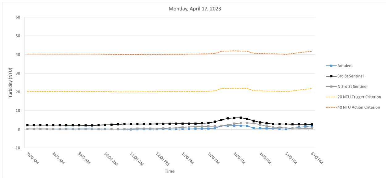
Figure 3. Hourly rolling average turbidity readings on Monday, April 17, 2023, from 7 AM to 6 PM.
