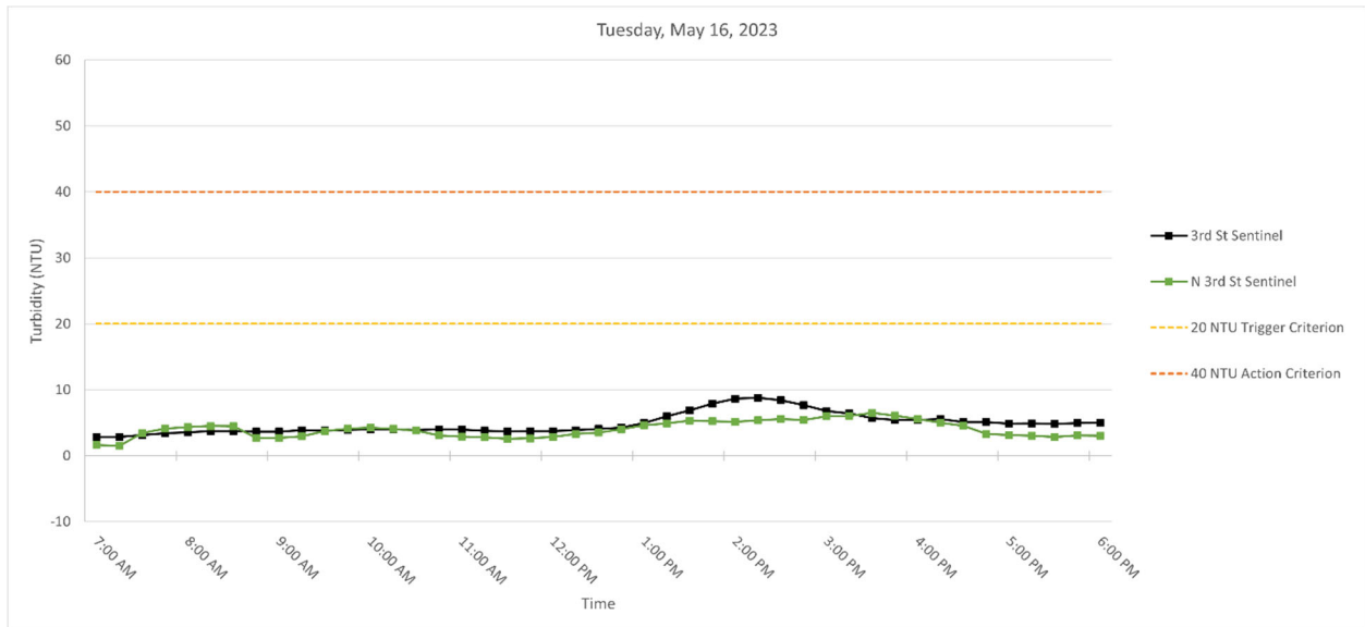
Figure 3. Hourly rolling average turbidity readings on Tuesday, May 16, 2023, from 7 AM to 6 PM.
