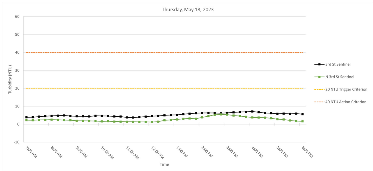
Figure 5. Hourly rolling average turbidity readings on Thursday, May 18, 2023, from 7 AM to 6 PM.
