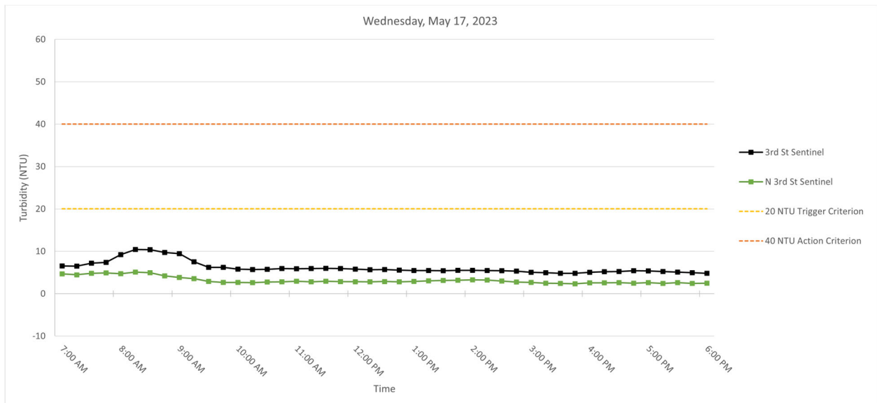
Figure 4. Hourly rolling average turbidity readings on Wednesday, May 17, 2023, from 7 AM to 6 PM.
