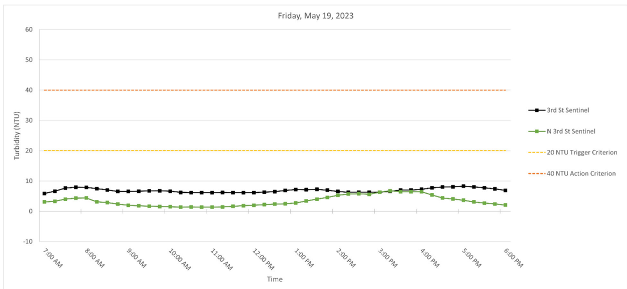
Figure 6. Hourly rolling average turbidity readings on Friday, May 19, 2023, from 7 AM to 6 PM.
