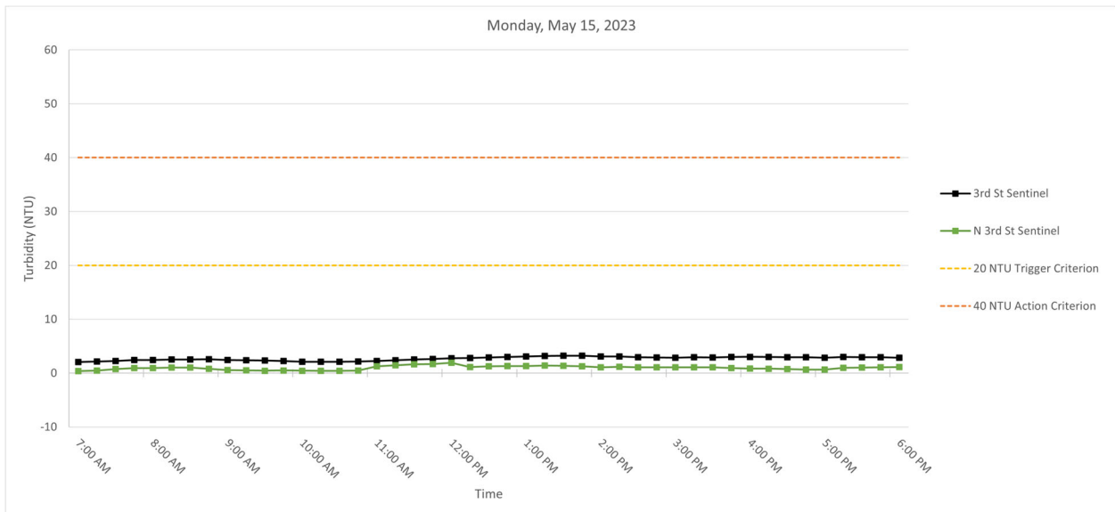
Figure 3. Hourly rolling average turbidity readings on Monday, May 15, 2023, from 7 AM to 6 PM.
