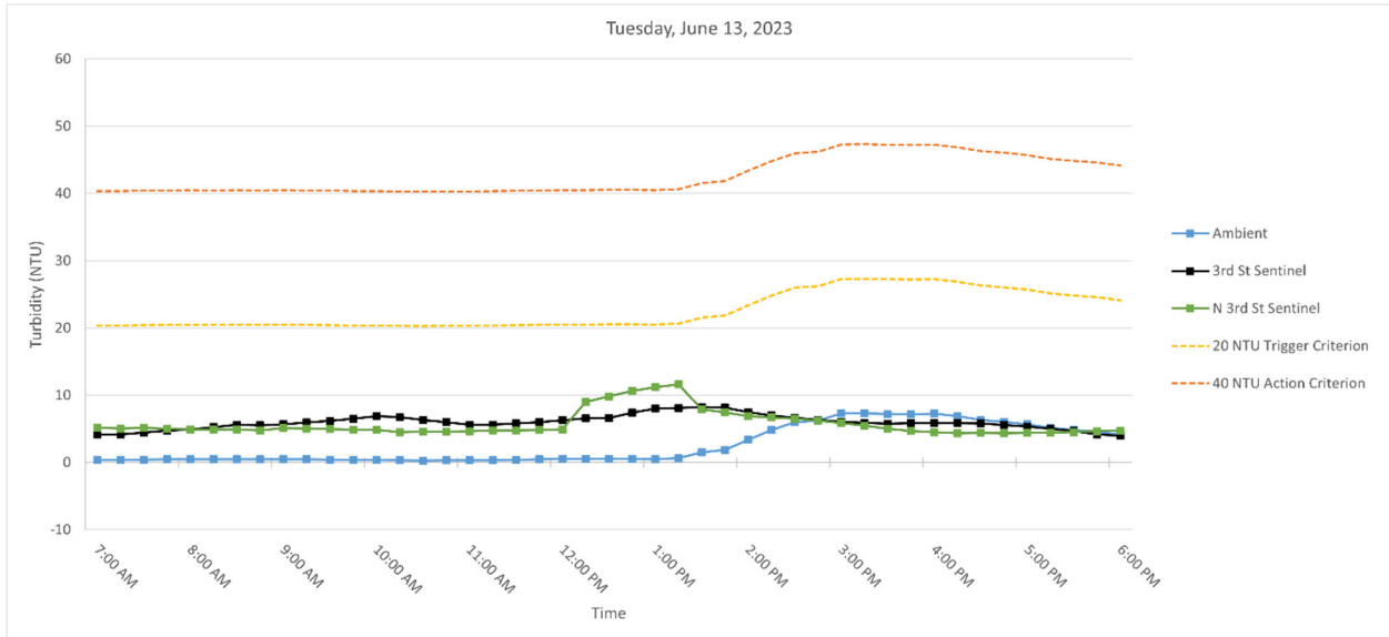
Figure 3. Hourly rolling average turbidity readings on Tuesday, June 13, 2023, from 7 AM to 6 PM.
