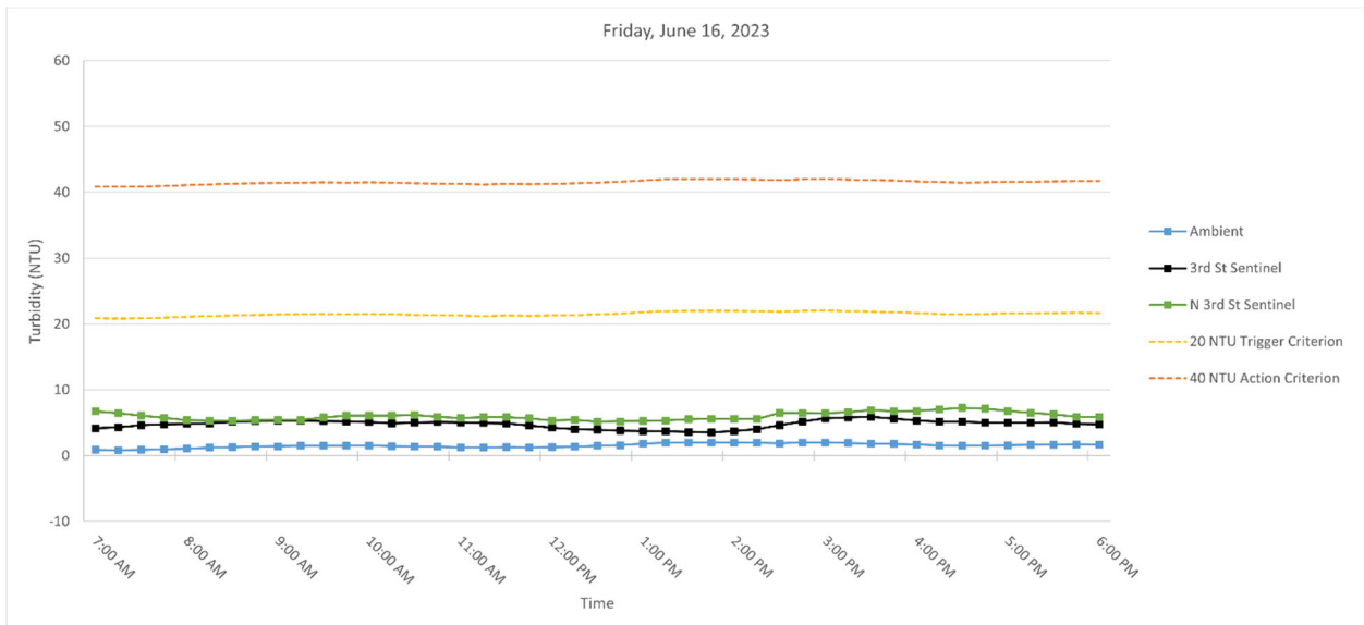
Figure 6. Hourly rolling average turbidity readings on Friday, June 16, 2023, from 7 AM to 6 PM.
