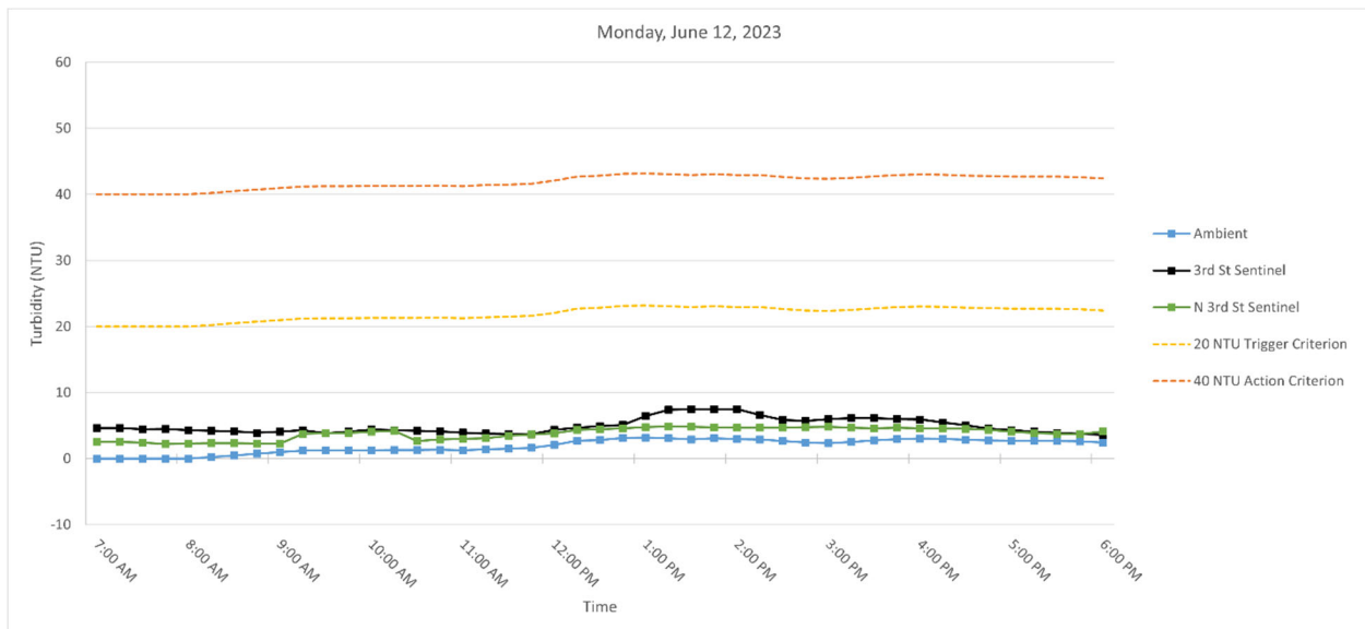
Figure 3. Hourly rolling average turbidity readings on Monday, June 12, 2023, from 7 AM to 6 PM.
