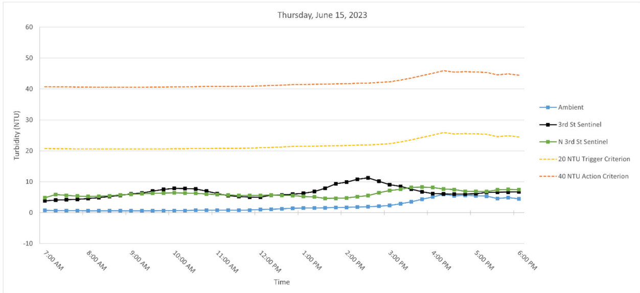
Figure 5. Hourly rolling average turbidity readings on Thursday, June 15, 2023, from 7 AM to 6 PM.
