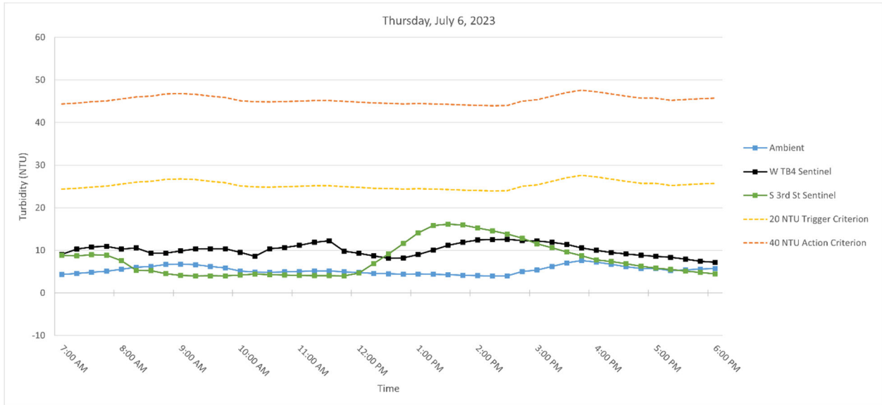
Figure 5. Hourly rolling average turbidity readings on Thursday, July 6, 2023, from 7 AM to 6 PM.
