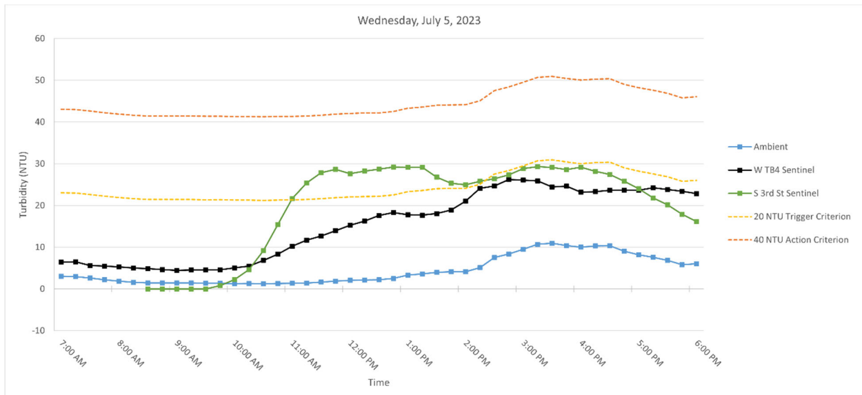
Figure 4. Hourly rolling average turbidity readings on Wednesday, July 5, 2023, from 7 AM to 6 PM.
