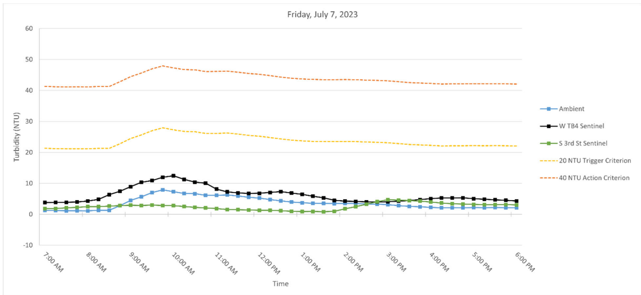
Figure 6. Hourly rolling average turbidity readings on Friday, July 7, 2023, from 7 AM to 6 PM.
