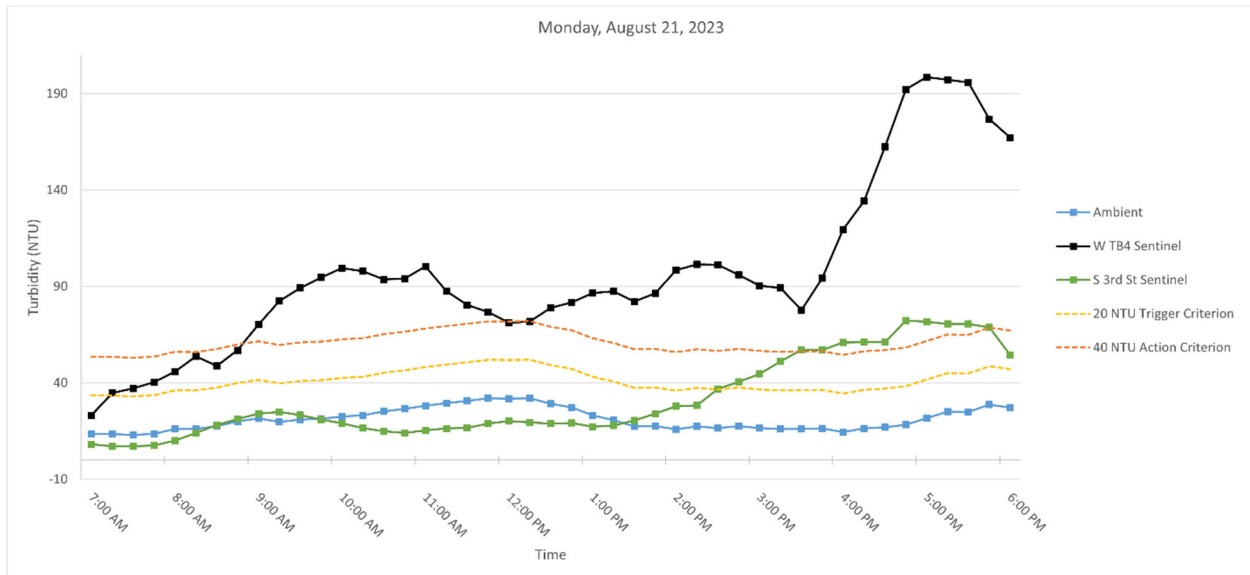
Figure 3. Hourly rolling average turbidity readings on Monday, August 21, 2023, from 7 AM to 6 PM.
