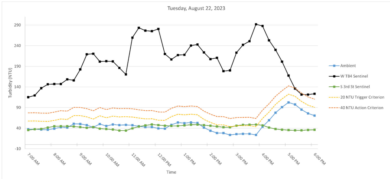
Figure 3. Hourly rolling average turbidity readings on Tuesday, August 22, 2023, from 7 AM to 6 PM.
