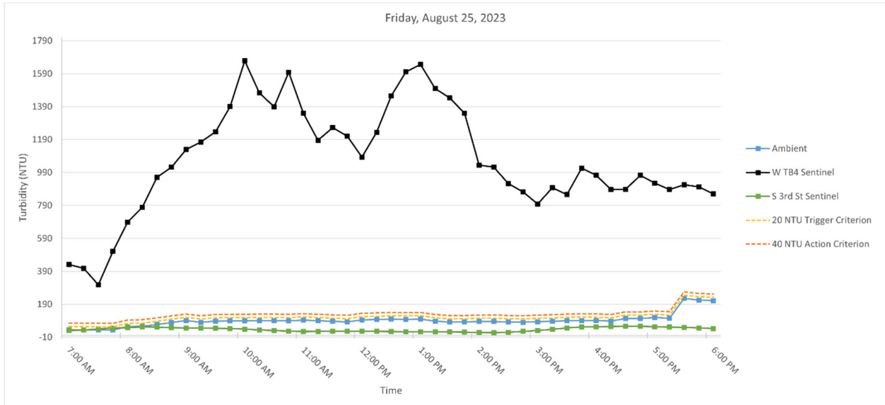
Figure 6. Hourly rolling average turbidity readings on Friday, August 25, 2023, from 7 AM to 6 PM.
