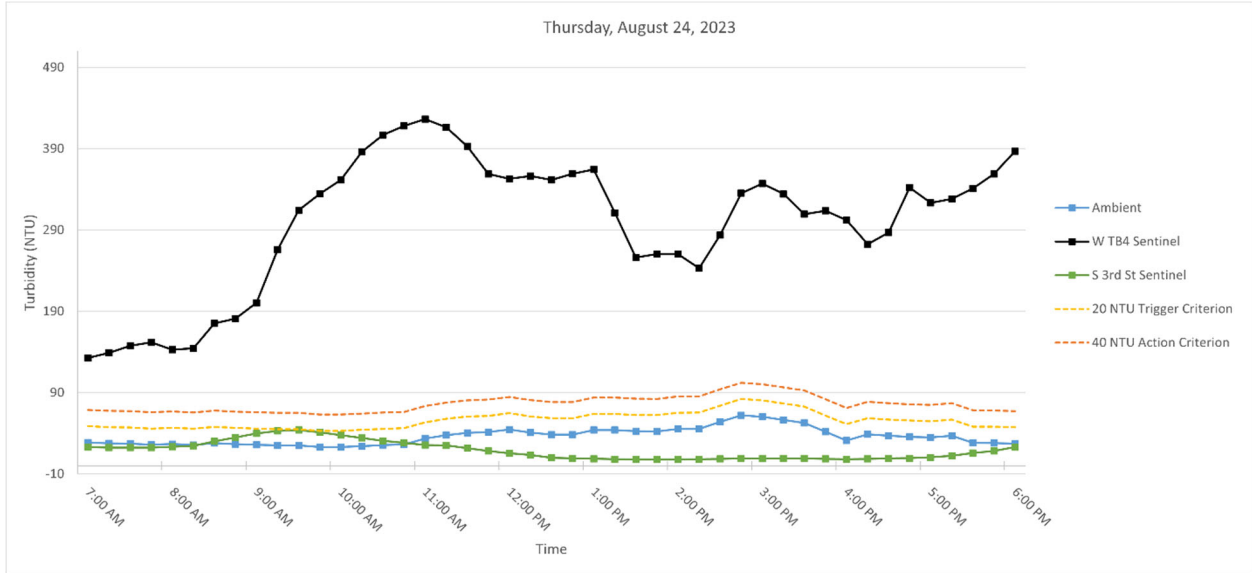
Figure 5. Hourly rolling average turbidity readings on Thursday, August 24, 2023, from 7 AM to 6 PM.
