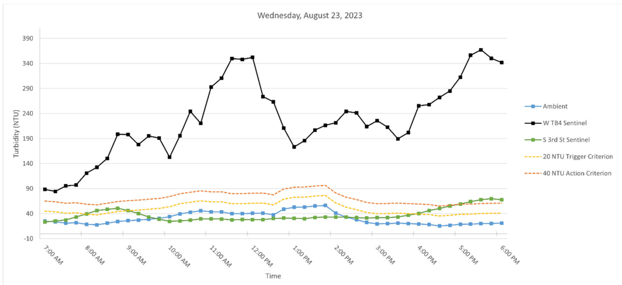
Figure 4. Hourly rolling average turbidity readings on Wednesday, August 23, 2023, from 7 AM to 6 PM.
