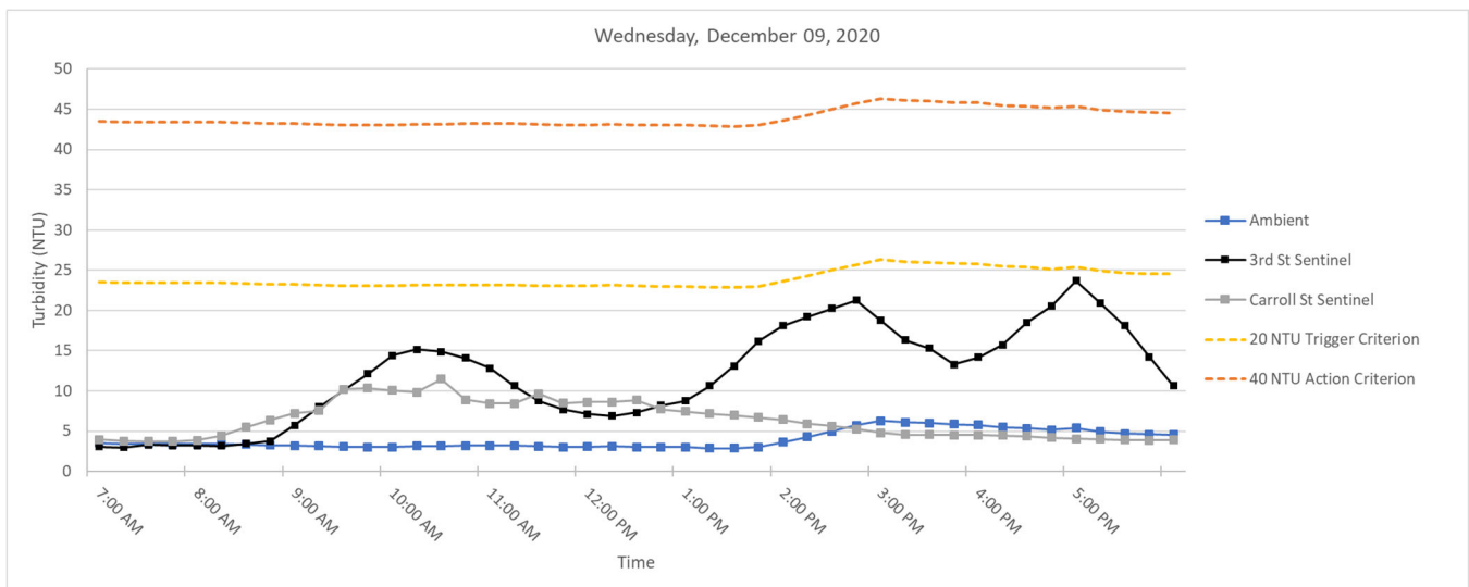
Figure 4. Hourly rolling average turbidity readings on Wednesday, December 09, 2020 from 7 AM to 6 PM.
