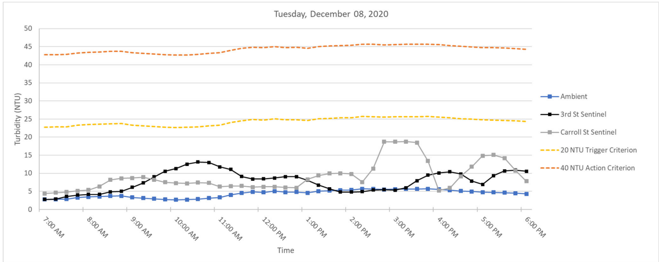
Figure 3. Hourly rolling average turbidity readings on Tuesday, December 08, 2020 from 7 AM to 6 PM.
