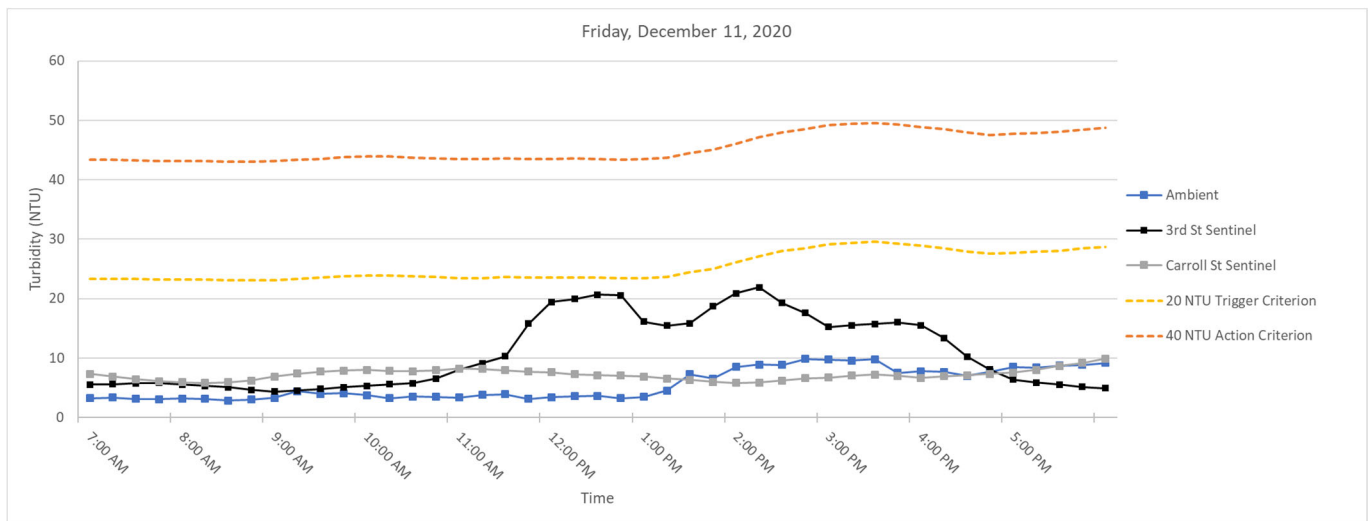
Figure 6. Hourly rolling average turbidity readings on Friday, December 11, 2020 from 7 AM to 6 PM.
