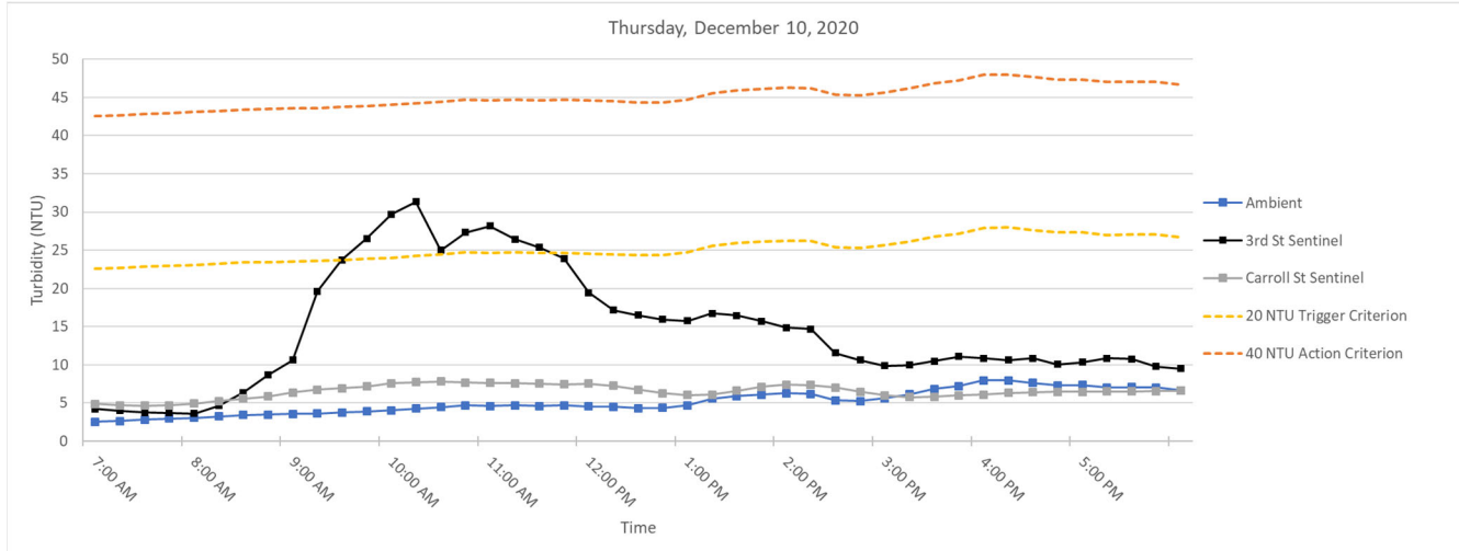
Figure 5. Hourly rolling average turbidity readings on Thursday, December 10, 2020 from 7 AM to 6 PM.
