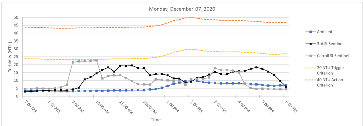
Figure 2. Hourly rolling average turbidity readings on Monday, December 07, 2020 from 7 AM to 6 PM.
