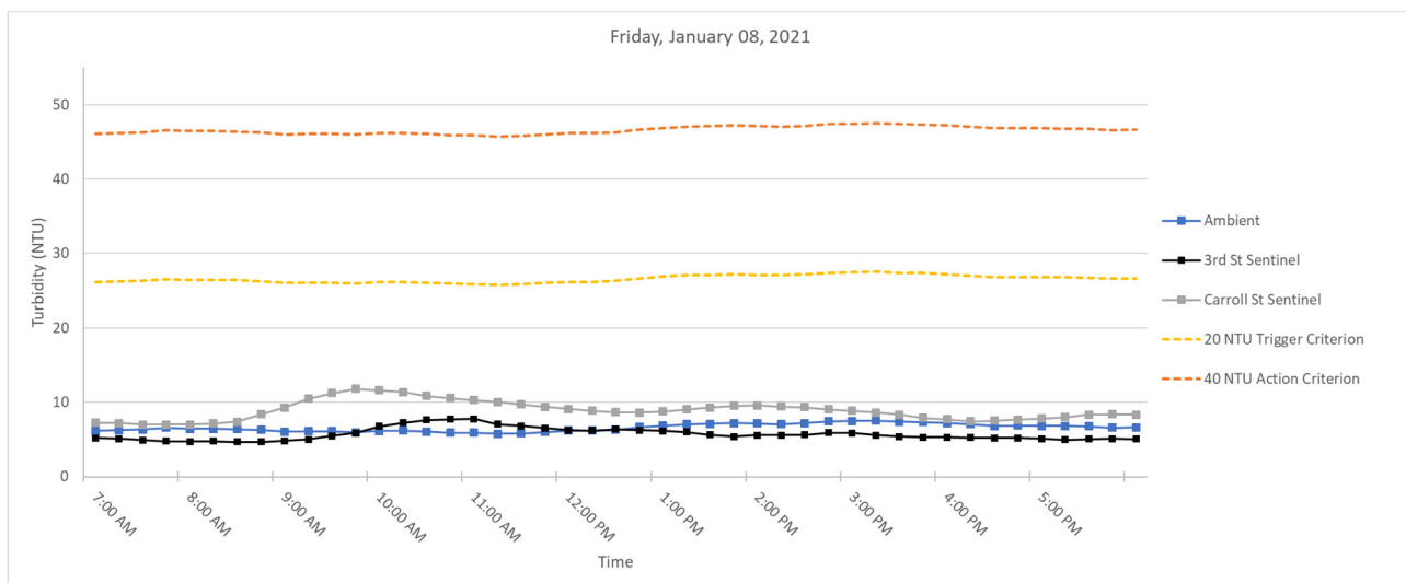
Figure 5. Hourly rolling average turbidity readings on Friday, January 08, 2021 from 7 AM to 6 PM.
