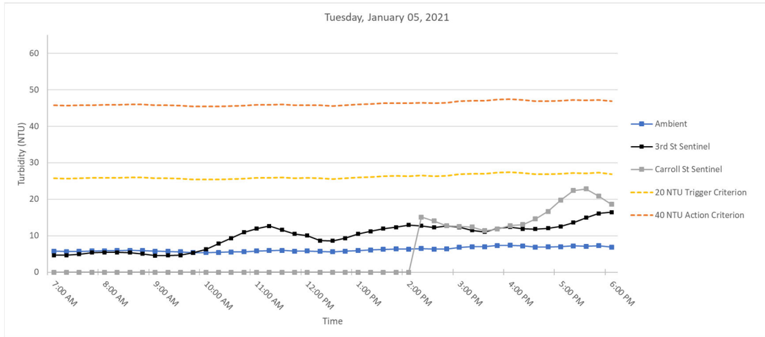
Figure 3. Hourly rolling average turbidity readings on Tuesday, January 05, 2021 from 7 AM to 6 PM.
