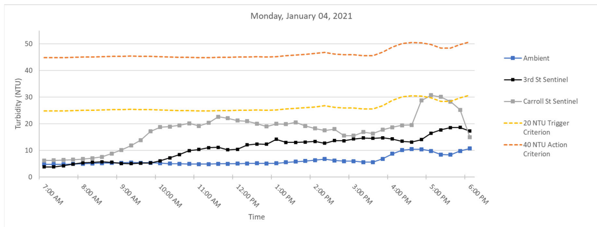
Figure 2. Hourly rolling average turbidity readings on Monday, January 04, 2021 from 7 AM to 6 PM.
