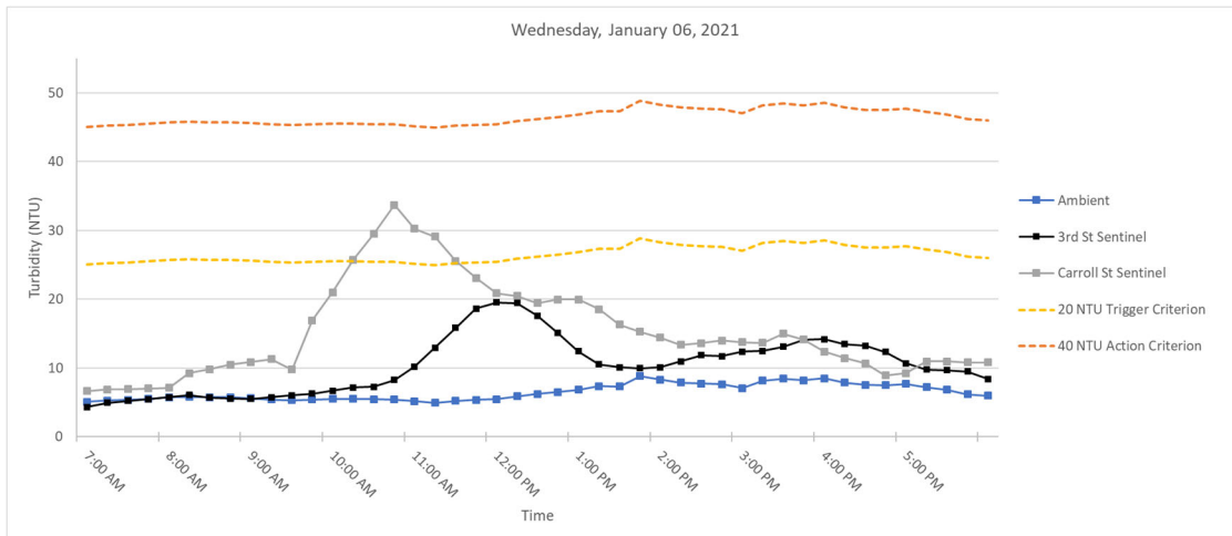
Figure 4. Hourly rolling average turbidity readings on Wednesday, January 06, 2021 from 7 AM to 6 PM.
