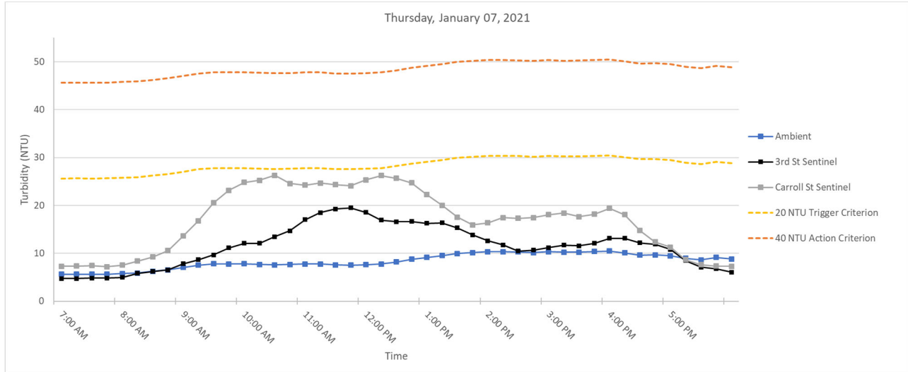
Figure 5. Hourly rolling average turbidity readings on Thursday, January 07, 2021 from 7 AM to 6 PM.
