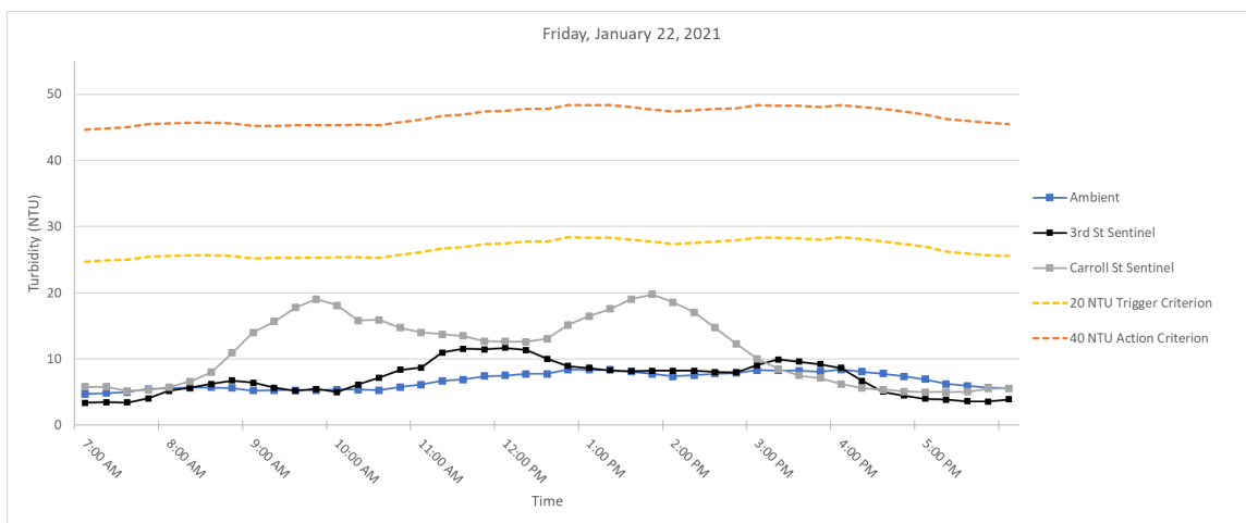
Figure 6. Hourly rolling average turbidity readings on Friday, January 22, 2021 from 7 AM to 6 PM.
