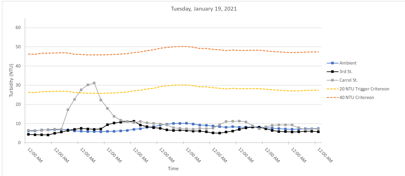
Figure 3. Hourly rolling average turbidity readings on Tuesday, January 19, 2021 from 7 AM to 6 PM.
