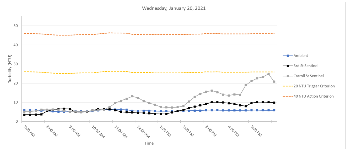
Figure 4. Hourly rolling average turbidity readings on Wednesday, January 20, 2021 from 7 AM to 6 PM.
