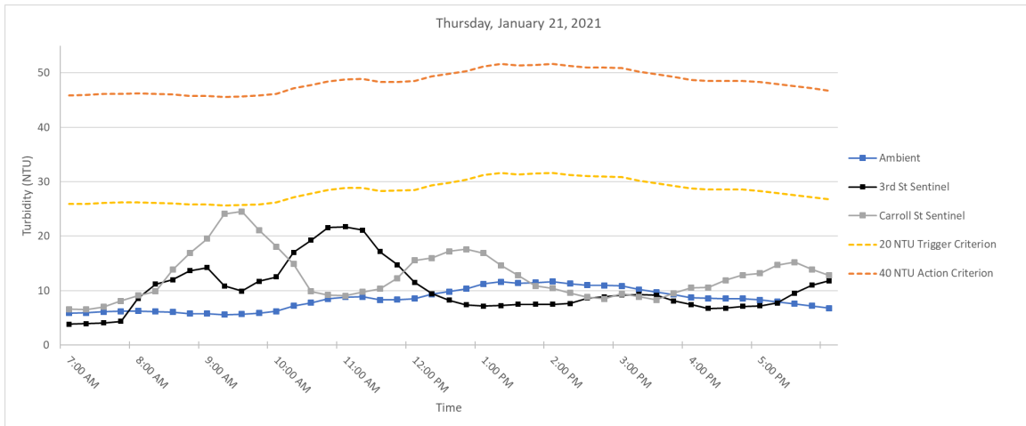
Figure 5. Hourly rolling average turbidity readings on Thursday, January 21, 2021 from 7 AM to 6 PM.
