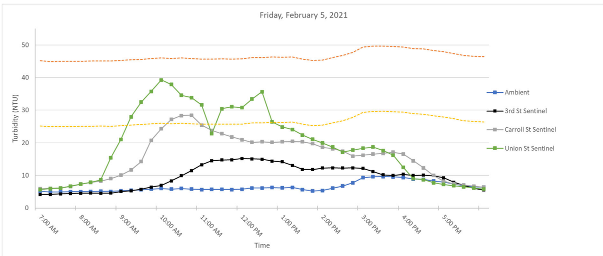
Figure 6. Hourly rolling average turbidity readings on Friday, February 5, 2021 from 7 AM to 6 PM.
