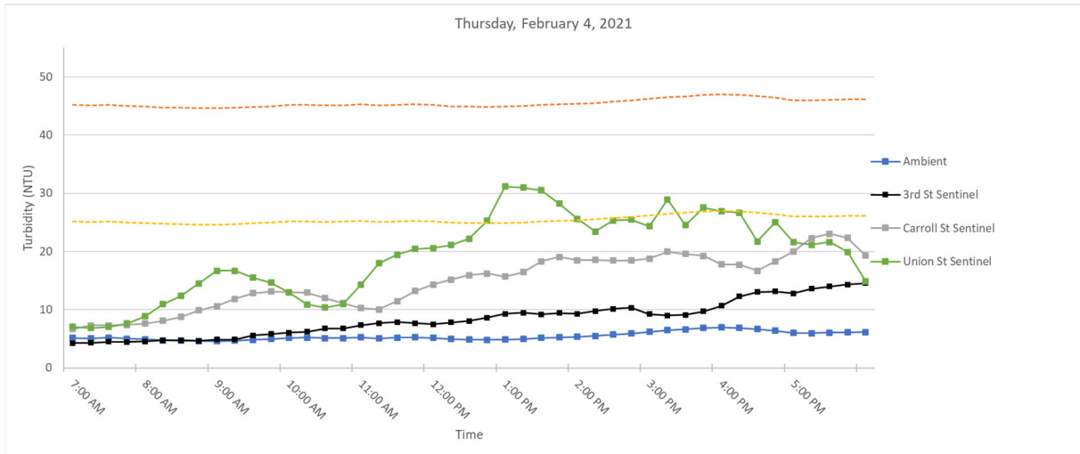
Figure 5. Hourly rolling average turbidity readings on Thursday, February 4, 2021 from 7 AM to 6 PM.
