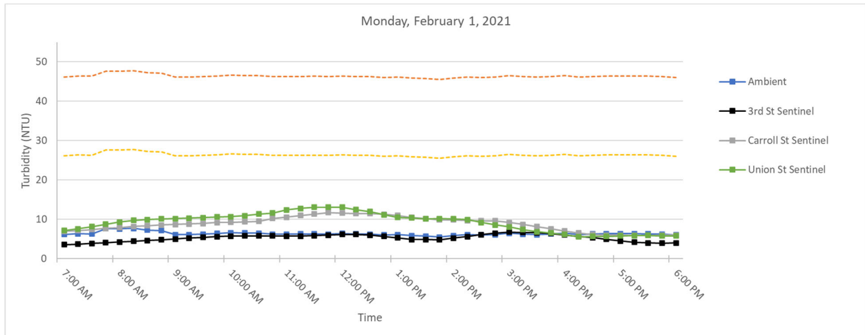
Figure 2. Hourly rolling average turbidity readings on Monday, February 1, 2021 from 7 AM to 6 PM.
