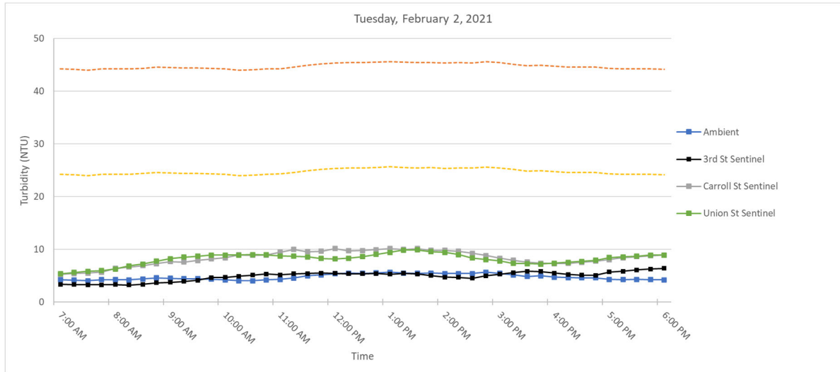
Figure 3. Hourly rolling average turbidity readings on Tuesday, February 2, 2021 from 7 AM to 6 PM.
