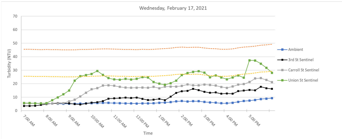
Figure 4. Hourly rolling average turbidity readings on Wednesday, February 17, 2021 from 7 AM to 6 PM.
