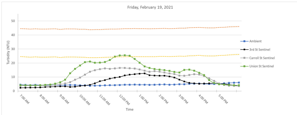
Figure 6. Hourly rolling average turbidity readings on Friday, February 19, 2021 from 7 AM to 6 PM.
