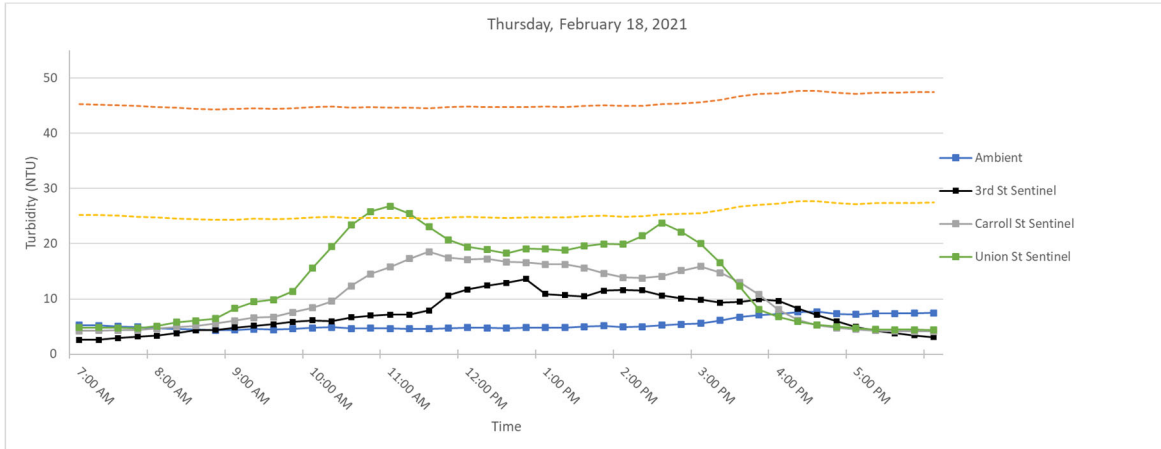
Figure 5. Hourly rolling average turbidity readings on Thursday, February 18, 2021 from 7 AM to 6 PM.
