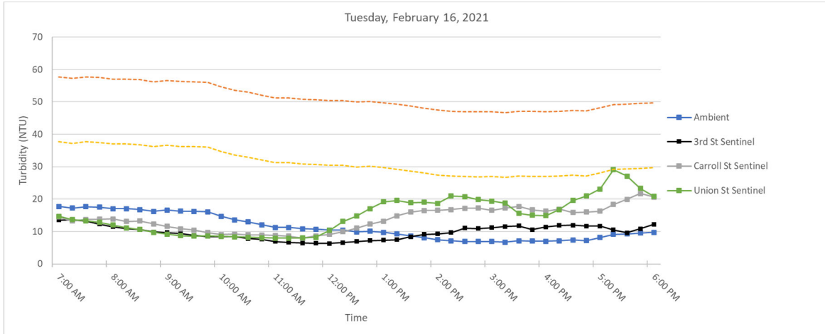
Figure 3. Hourly rolling average turbidity readings on Tuesday, February 16, 2021 from 7 AM to 6 PM.
