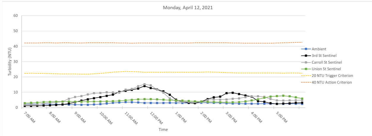
Figure 2. Hourly rolling average turbidity readings on Monday, April 12, 2021 from 7 AM to 6 PM.
