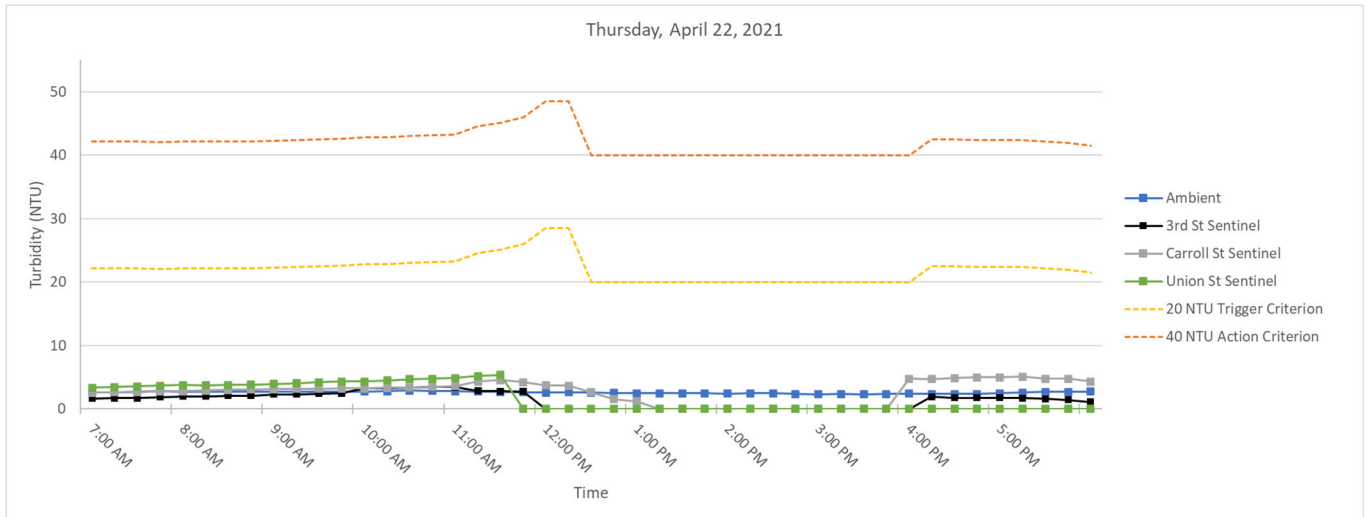
Figure 5. Hourly rolling average turbidity readings on Thursday, April 22, 2021 from 7 AM to 6 PM.
