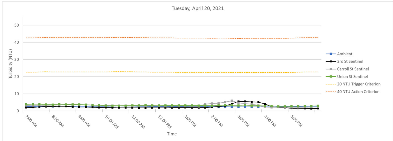
Figure 3. Hourly rolling average turbidity readings on Tuesday, April 20, 2021 from 7 AM to 6 PM.
