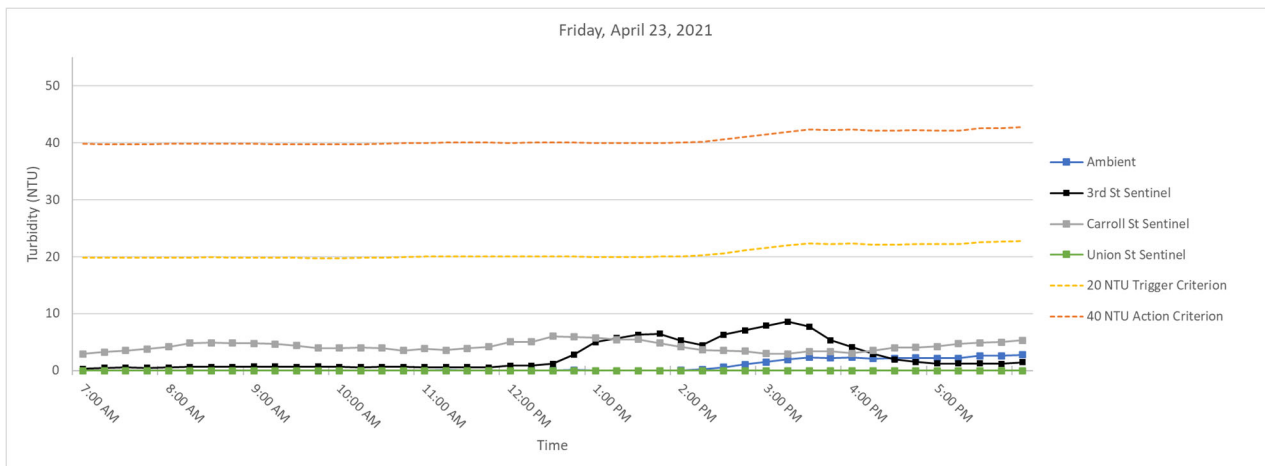
Figure 6. Hourly rolling average turbidity readings on Friday, April 23, 2021 from 7 AM to 6 PM.
