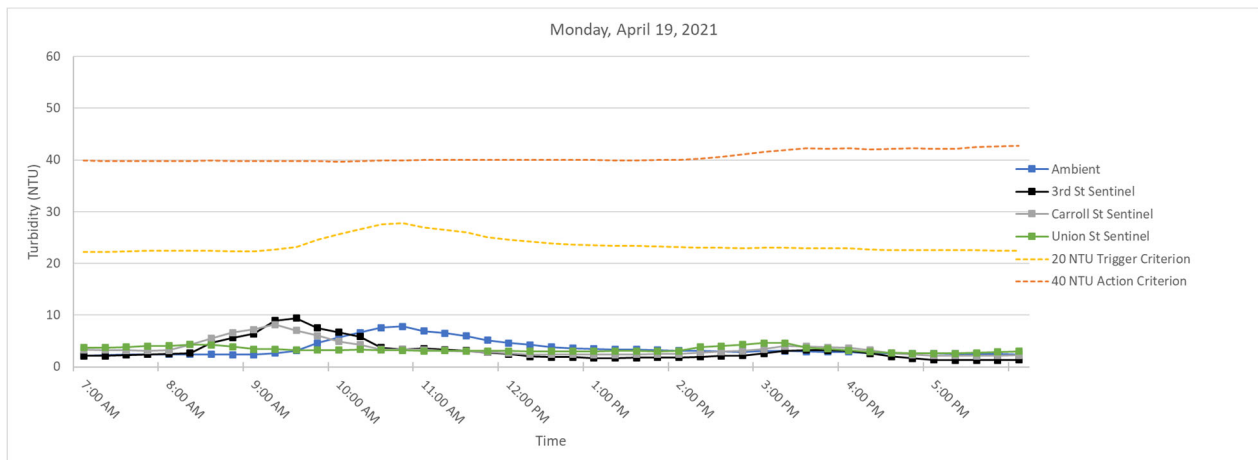
Figure 2. Hourly rolling average turbidity readings on Monday, April 19, 2021 from 7 AM to 6 PM.
