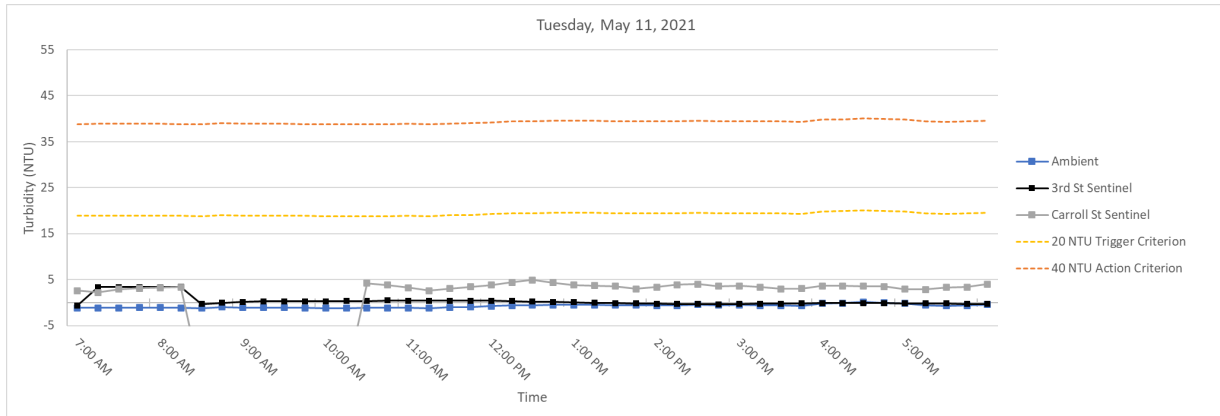
Figure 3. Hourly rolling average turbidity readings on Tuesday, May 11, 2021 from 7 AM to 6 PM.
