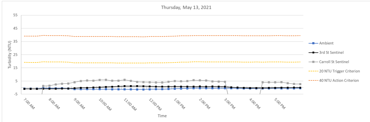
Figure 5. Hourly rolling average turbidity readings on Thursday, May 13, 2021 from 7 AM to 6 PM.
