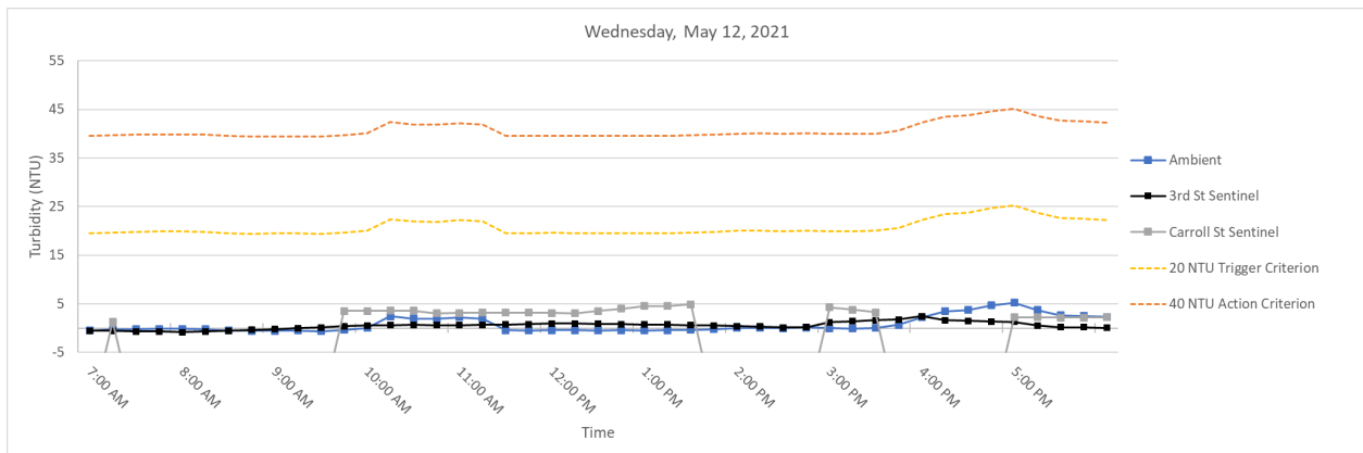
Figure 4. Hourly rolling average turbidity readings on Wednesday, May 12, 2021 from 7 AM to 6 PM.
