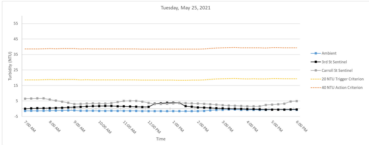
Figure 3. Hourly rolling average turbidity readings on Tuesday, May 25, 2021 from 7 AM to 6 PM.
