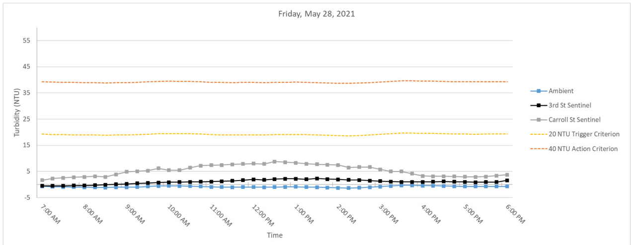
Figure 6. Hourly rolling average turbidity readings on Friday, May 28, 2021 from 7 AM to 6 PM.
