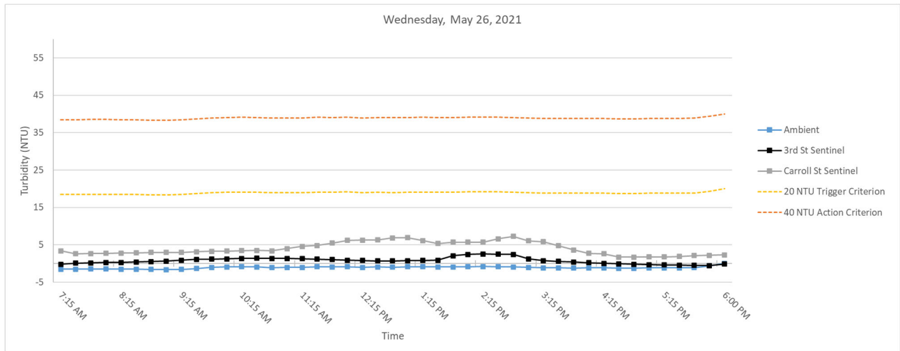
Figure 4. Hourly rolling average turbidity readings on Wednesday, May 26, 2021 from 7 AM to 6 PM.
