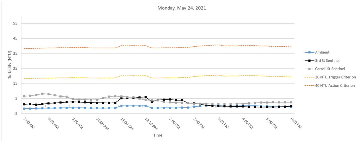
Figure 2. Hourly rolling average turbidity readings on Monday, May 24, 2021 from 7 AM to 6 PM.
