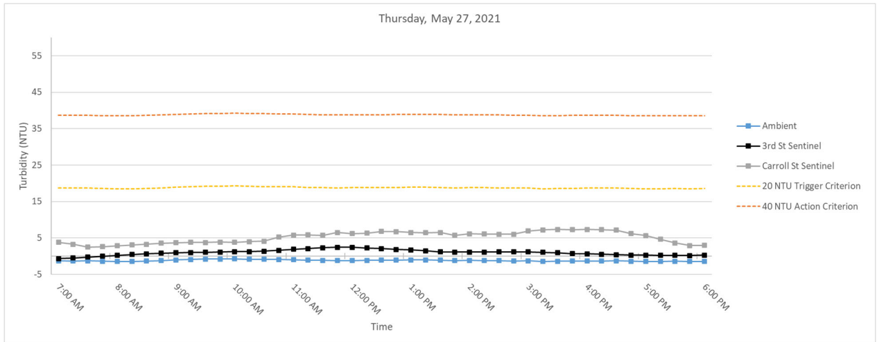
Figure 5. Hourly rolling average turbidity readings on Thursday, May 27, 2021 from 7 AM to 6 PM.
