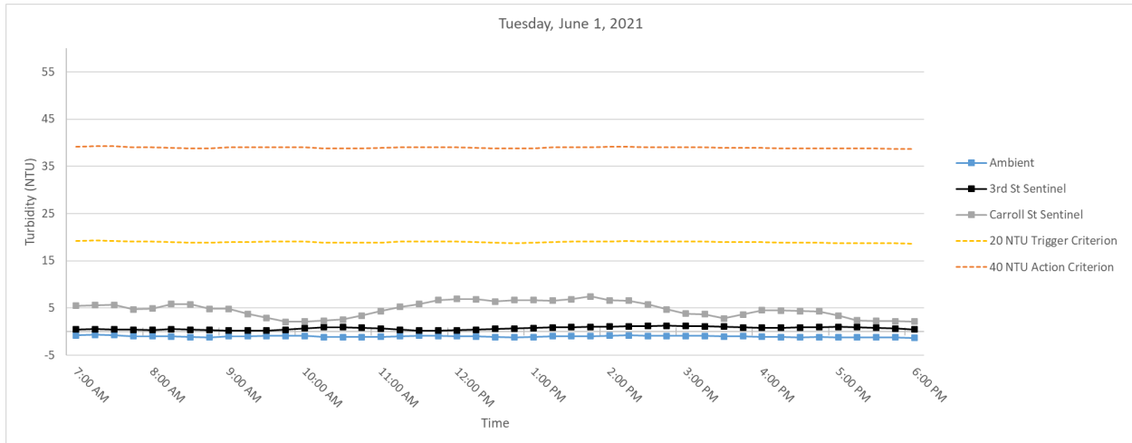
Figure 3. Hourly rolling average turbidity readings on Tuesday, June 1, 2021 from 7 AM to 6 PM.
