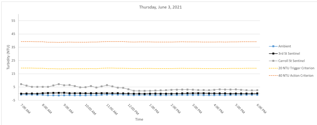
Figure 5. Hourly rolling average turbidity readings on Thursday, June 3, 2021 from 7 AM to 6 PM.
