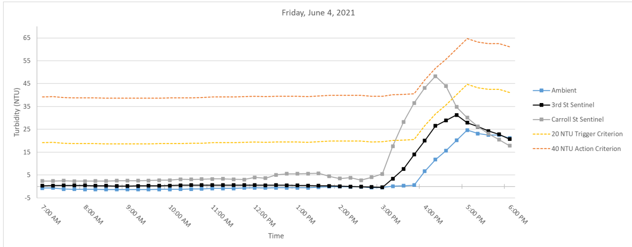
Figure 6. Hourly rolling average turbidity readings on Friday, June 4, 2021 from 7 AM to 6 PM.
