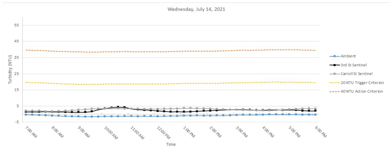
Figure 4. Hourly rolling average turbidity readings on Wednesday, July 14, 2021 from 7 AM to 6 PM.
