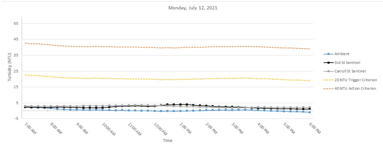
Figure 2. Hourly rolling average turbidity readings on Monday, July 12, 2021 from 7 AM to 6 PM.
