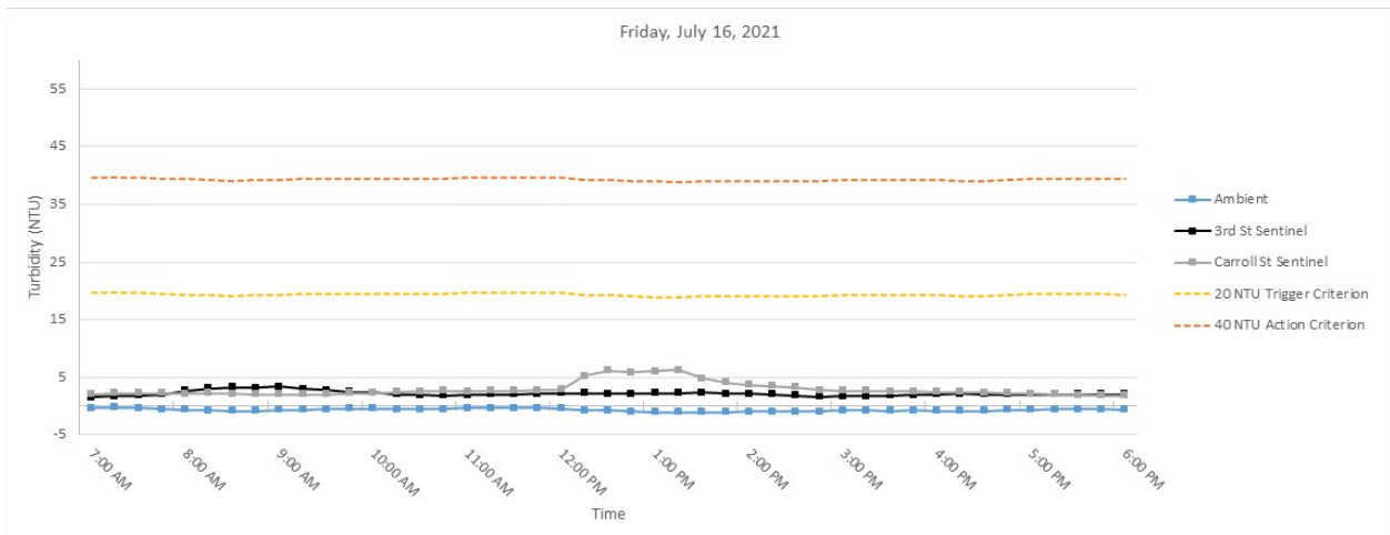
Figure 6. Hourly rolling average turbidity readings on Friday, July 16, 2021 from 7 AM to 6 PM.
