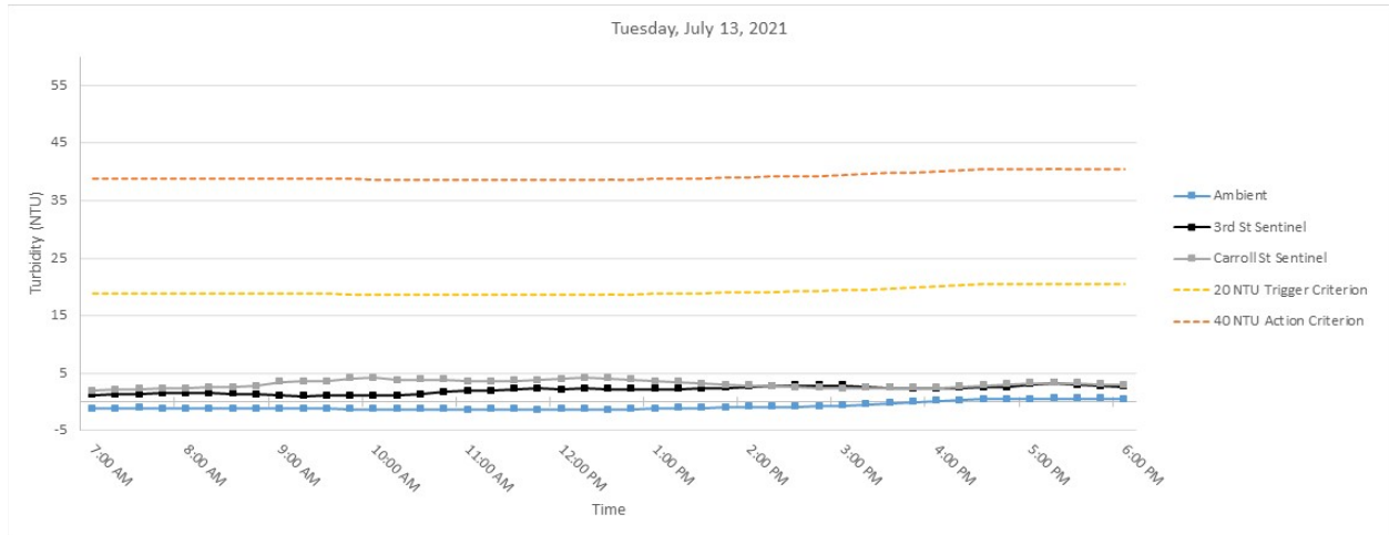
Figure 3. Hourly rolling average turbidity readings on Tuesday, July 13, 2021 from 7 AM to 6 PM.
