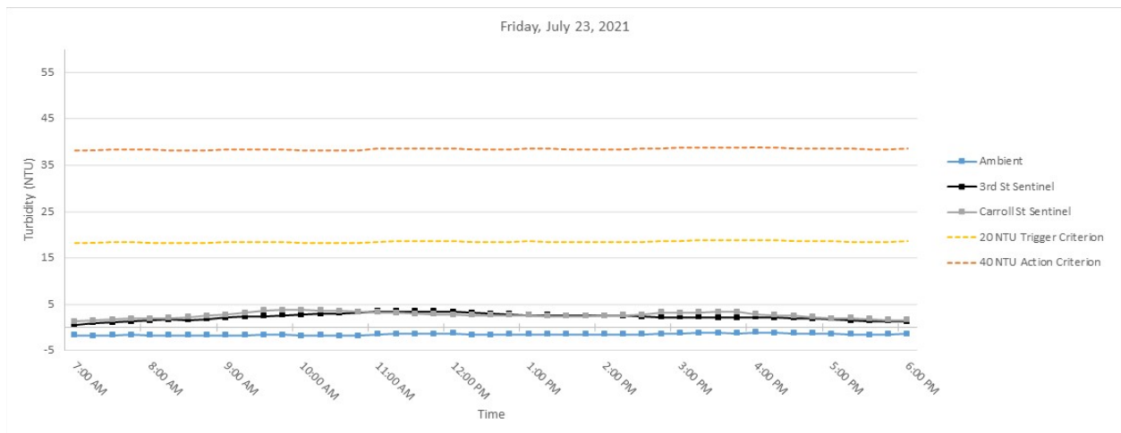
Figure 6. Hourly rolling average turbidity readings on Friday, July 23, 2021 from 7 AM to 6 PM.
