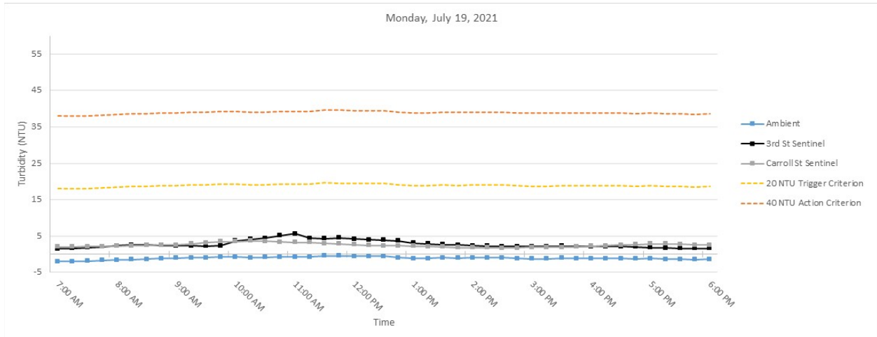
Figure 2. Hourly rolling average turbidity readings on Monday, July 19, 2021 from 7 AM to 6 PM.
