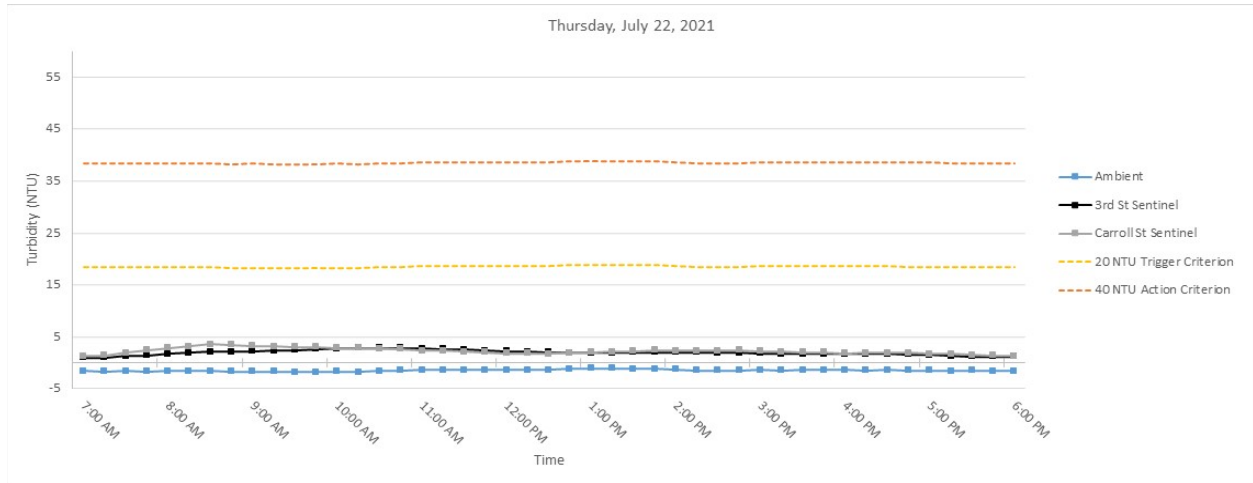
Figure 5. Hourly rolling average turbidity readings on Thursday, July 22, 2021 from 7 AM to 6 PM.
