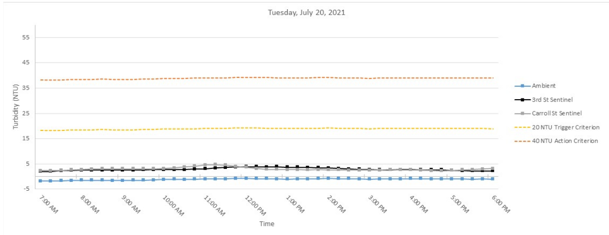
Figure 3. Hourly rolling average turbidity readings on Tuesday, July 20, 2021 from 7 AM to 6 PM.
