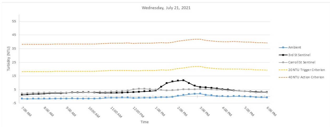
Figure 4. Hourly rolling average turbidity readings on Wednesday, July 21, 2021 from 7 AM to 6 PM.
