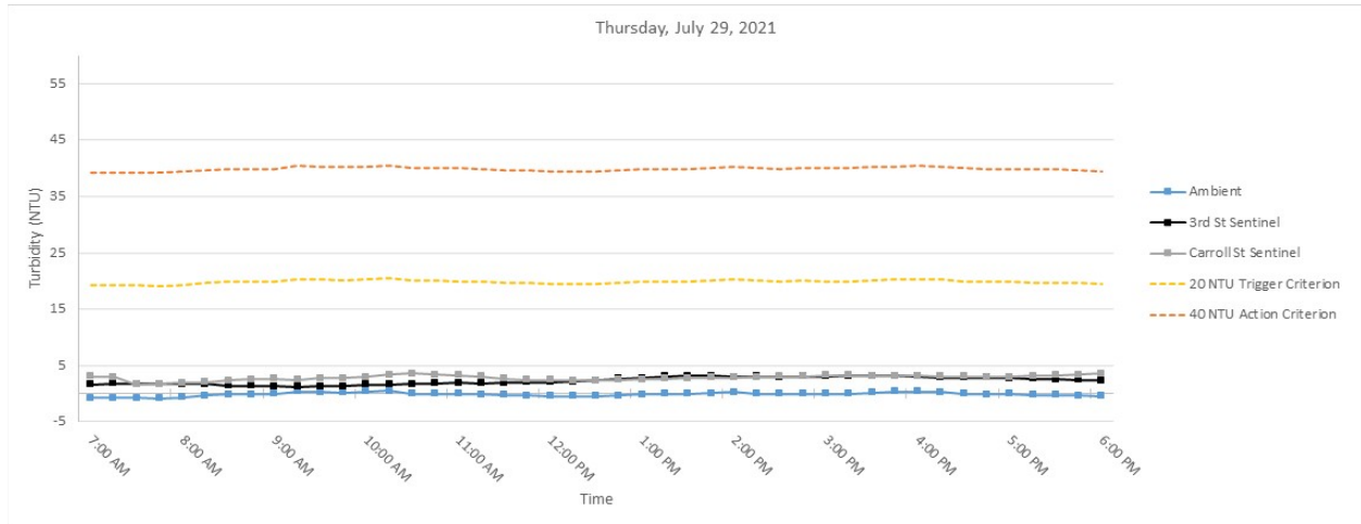
Figure 5. Hourly rolling average turbidity readings on Thursday, July 29, 2021 from 7 AM to 6 PM.
