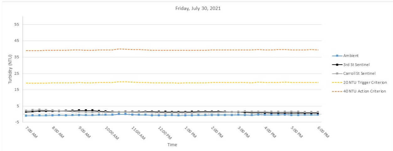
Figure 6. Hourly rolling average turbidity readings on Friday, July 30, 2021 from 7 AM to 6 PM.
