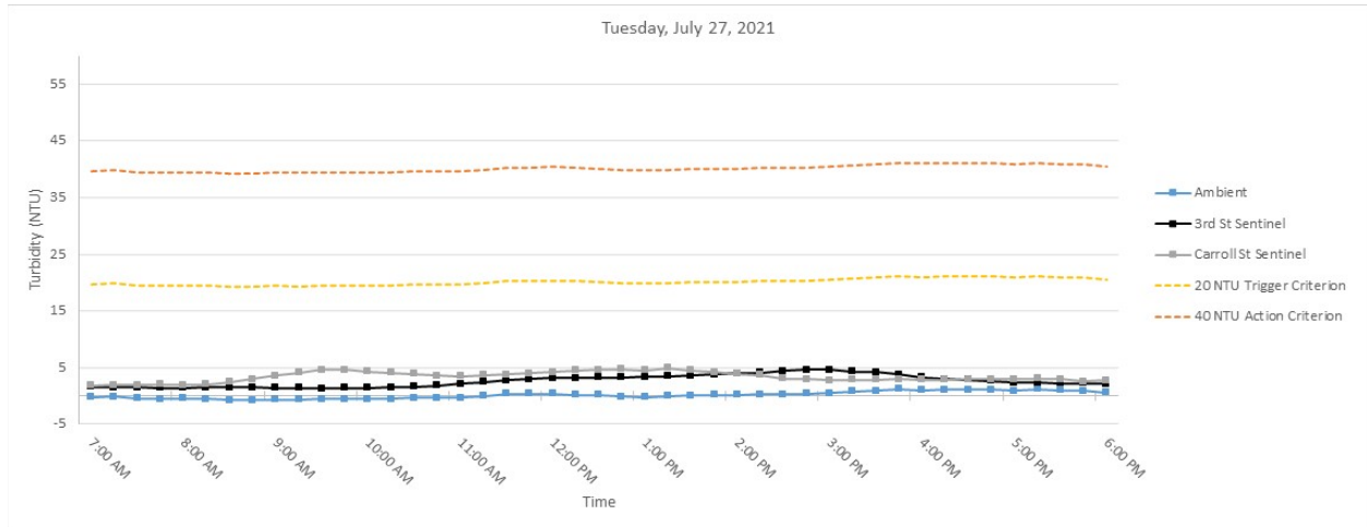
Figure 3. Hourly rolling average turbidity readings on Tuesday, July 27, 2021 from 7 AM to 6 PM.
