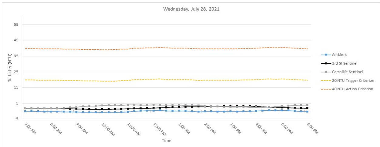
Figure 4. Hourly rolling average turbidity readings on Wednesday, July 28, 2021 from 7 AM to 6 PM.
