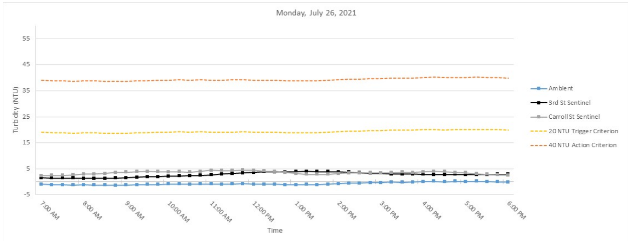
Figure 2. Hourly rolling average turbidity readings on Monday, July 26, 2021 from 7 AM to 6 PM.
