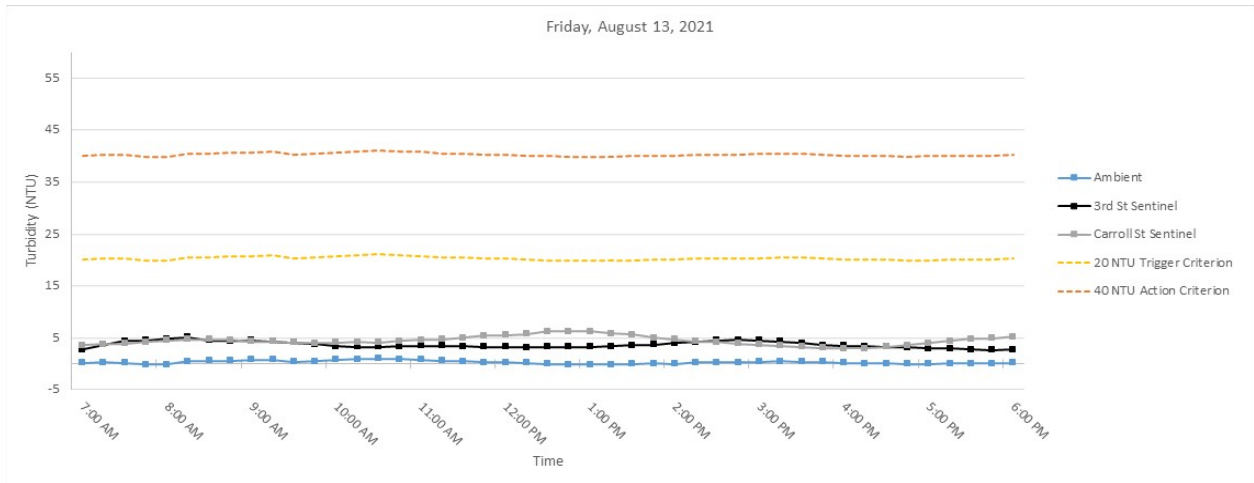
Figure 6. Hourly rolling average turbidity readings on Friday, August 13, 2021 from 7 AM to 6 PM.
