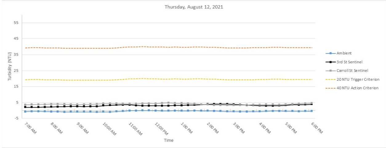
Figure 5. Hourly rolling average turbidity readings on Thursday, August 12, 2021 from 7 AM to 6 PM.
