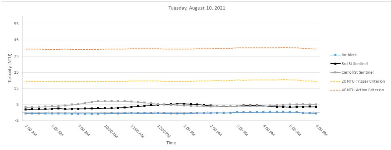
Figure 3. Hourly rolling average turbidity readings on Tuesday, August 10, 2021 from 7 AM to 6 PM.
