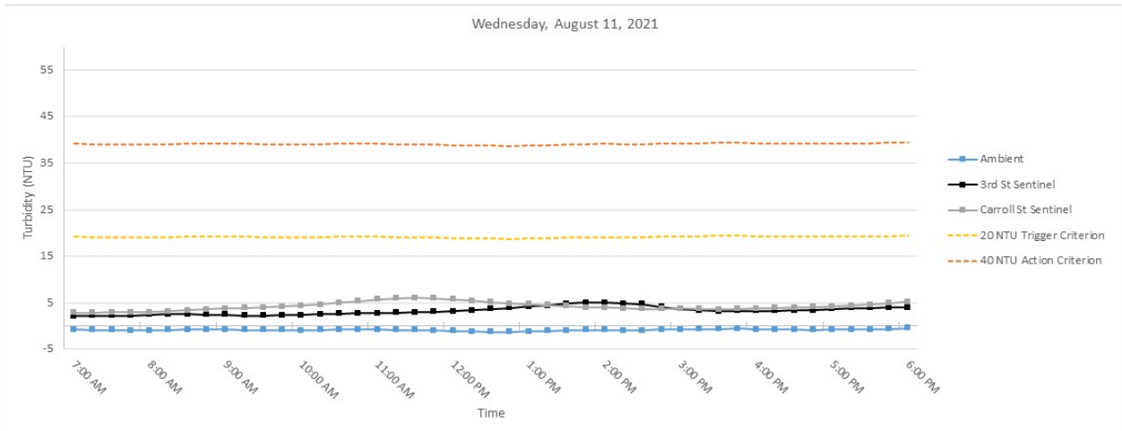
Figure 4. Hourly rolling average turbidity readings on Wednesday, August 11, 2021 from 7 AM to 6 PM.
