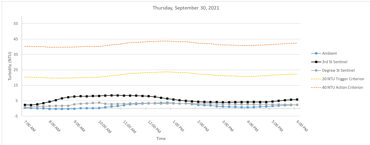
Figure 5. Hourly rolling average turbidity readings on Thursday, September 30, 2021 from 7 AM to 6 PM.
