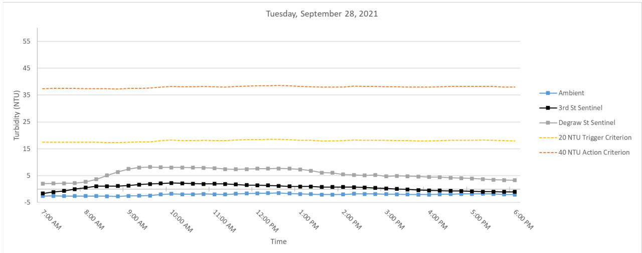
Figure 3. Hourly rolling average turbidity readings on Tuesday, September 28, 2021 from 7 AM to 6 PM.
