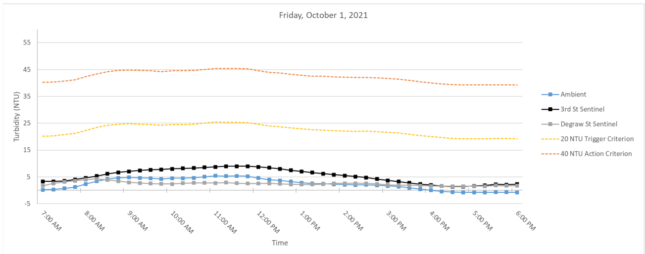
Figure 6. Hourly rolling average turbidity readings on Friday, October 1, 2021 from 7 AM to 6 PM.
