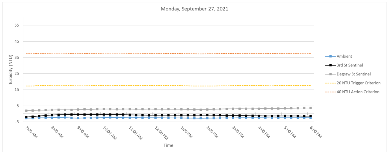
Figure 2. Hourly rolling average turbidity readings on Monday, September 27, 2021 from 7 AM to 6 PM.
