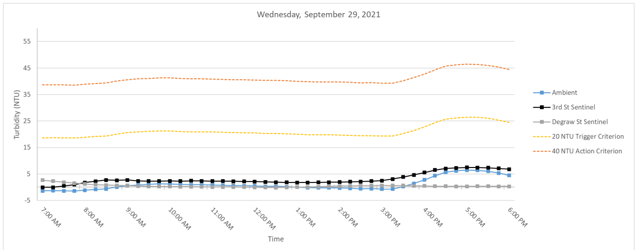
Figure 4. Hourly rolling average turbidity readings on Wednesday, September 29, 2021 from 7 AM to 6 PM.
