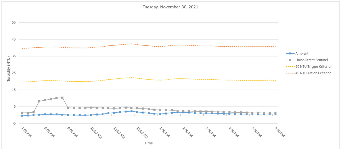
Figure 3. Hourly rolling average turbidity readings on Tuesday, November 30, 2021 from 7 AM to 6 PM.
