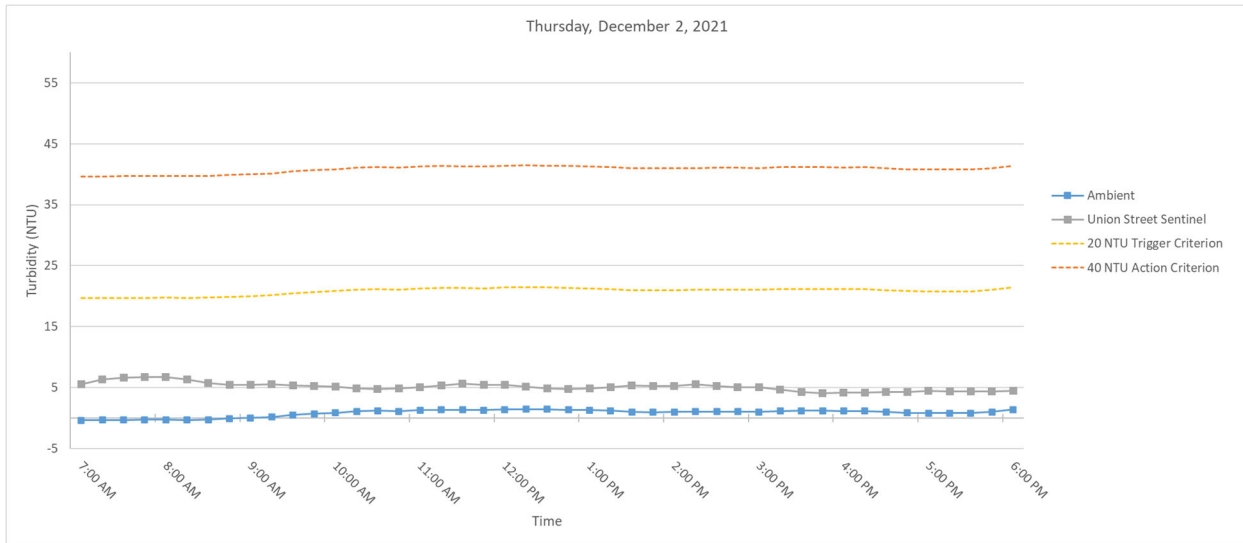
Figure 5. Hourly rolling average turbidity readings on Thursday, December 2, 2021 from 7 AM to 6 PM.
