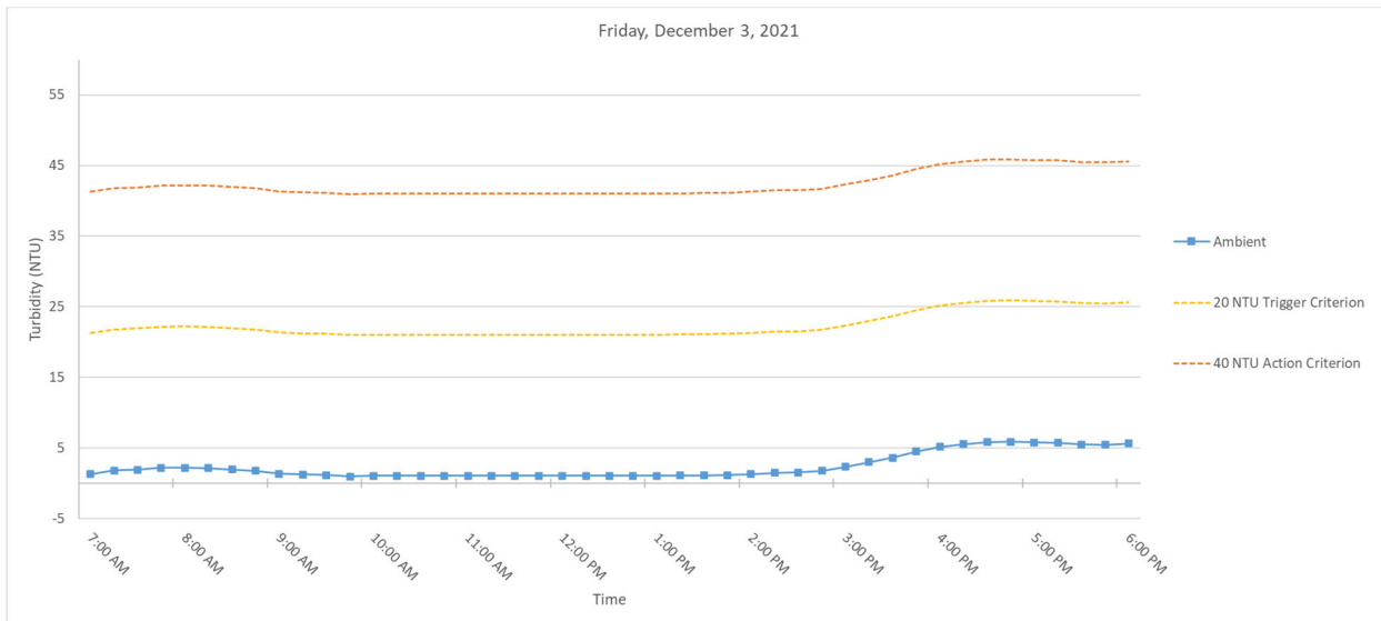
Figure 6. Hourly rolling average turbidity readings on Friday, December 3, 2021 from 7 AM to 6 PM.
