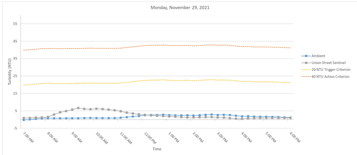
Figure 2. Hourly rolling average turbidity readings on Monday, November 29, 2021 from 7 AM to 6 PM.
